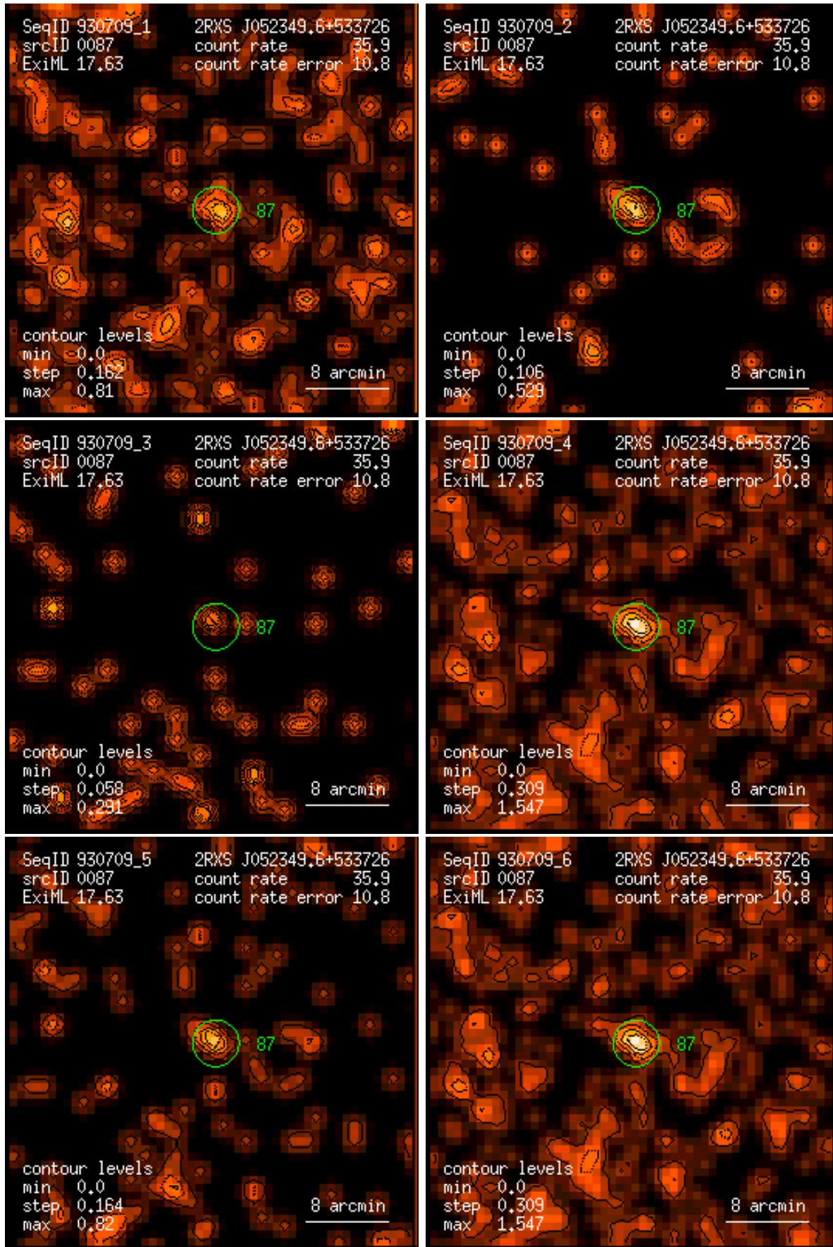
Figure 87: RASS 930709: detection 0087: band rate images, Gaussian filter: (1) PSPC channels 11 – 41, (2) 52 – 90, (3) 91 – 201, (4) 11 – 235, (5) 52 – 201, (6) 11 – 201. Broad band rates in counts/ks. Band rate contour levels in counts/ks/arcmin 2 .
