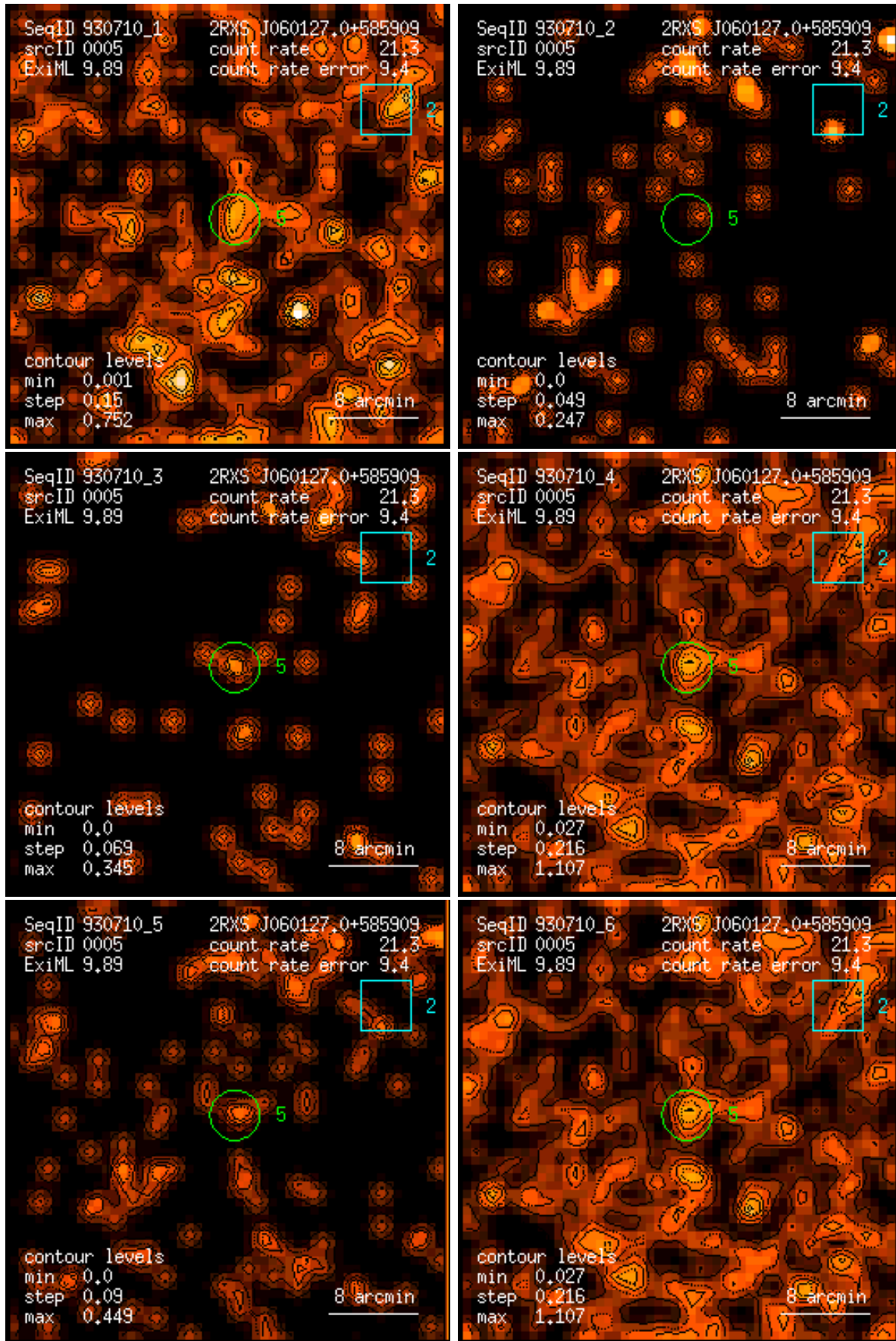
Figure 5: RASS 930710: detection 0005: band rate images, Gaussian filter: (1) PSPC channels 11 – 41, (2) 52 – 90, (3) 91 – 201, (4) 11 – 235, (5) 52 – 201, (6) 11 – 201. Broad band rates in counts/ks. Band rate contour levels in counts/ks/arcmin 2 .
