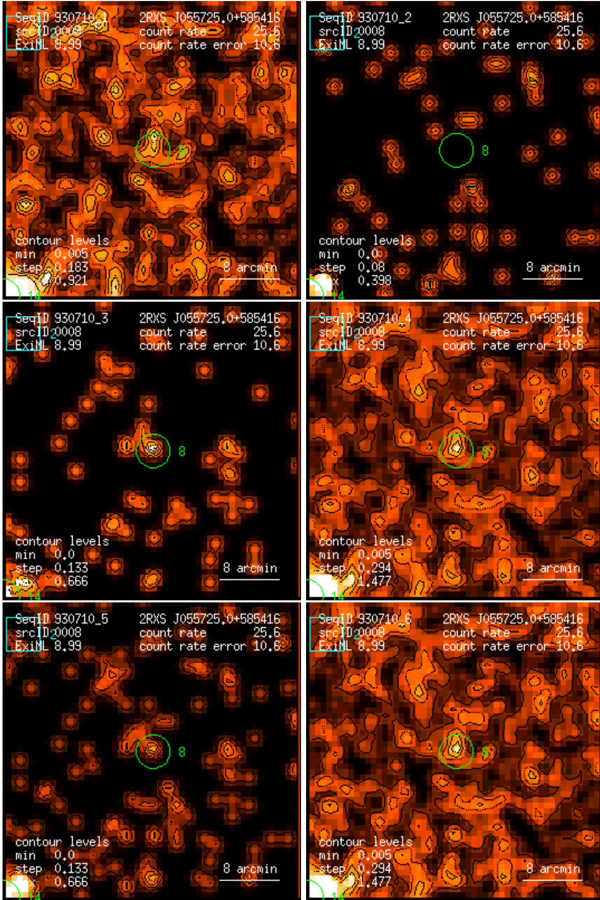
Figure 8: RASS 930710: detection 0008: band rate images, Gaussian filter: (1) PSPC channels 11 – 41, (2) 52 – 90, (3) 91 – 201, (4) 11 – 235, (5) 52 – 201, (6) 11 – 201. Broad band rates in counts/ks. Band rate contour levels in counts/ks/arcmin 2 .
