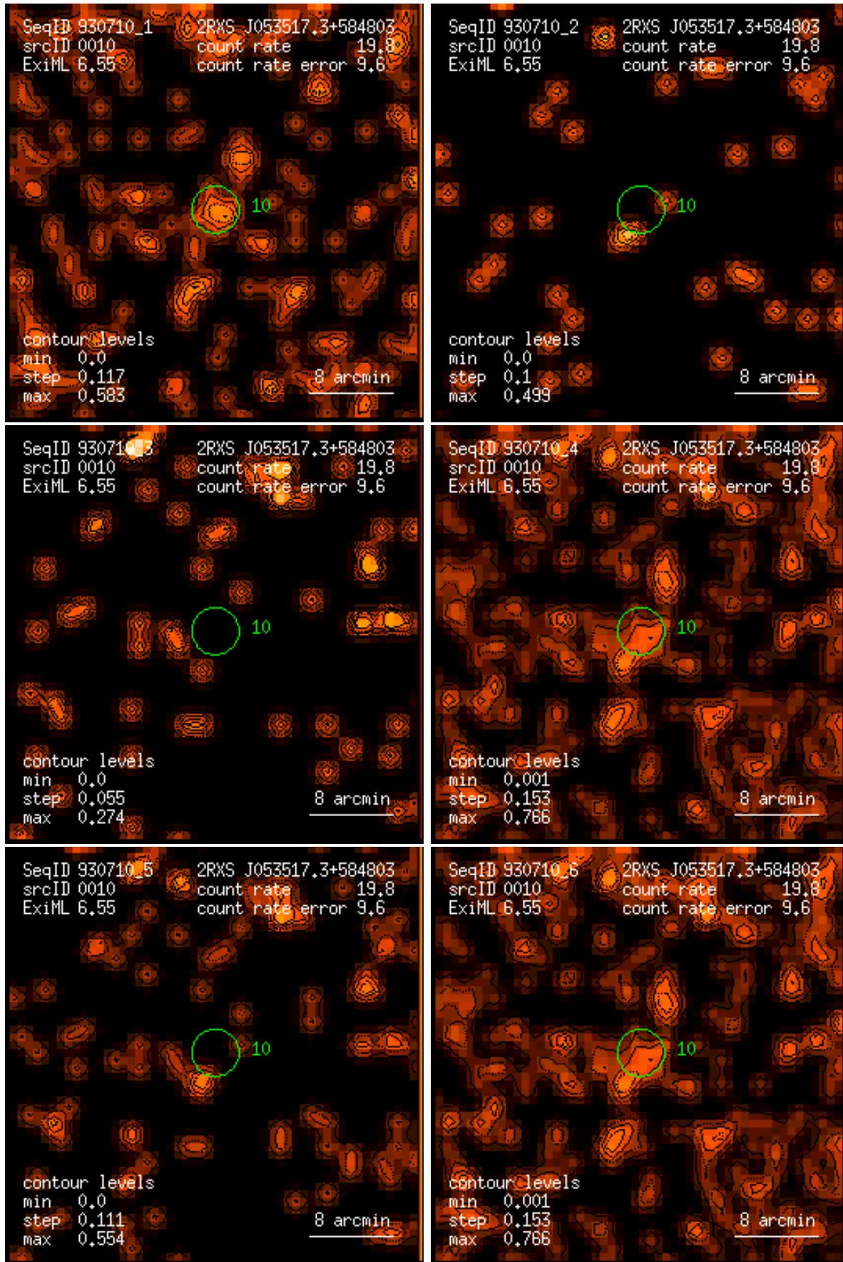
Figure 10: RASS 930710: detection 0010: band rate images, Gaussian filter: (1) PSPC channels 11 – 41, (2) 52 – 90, (3) 91 – 201, (4) 11 – 235, (5) 52 – 201, (6) 11 – 201. Broad band rates in counts/ks. Band rate contour levels in counts/ks/arcmin 2 .
