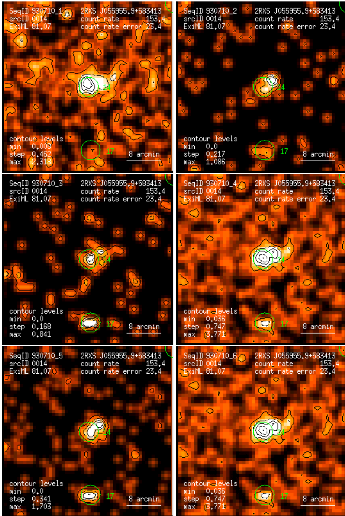
Figure 14: RASS 930710: detection 0014: band rate images, Gaussian filter: (1) PSPC channels 11 – 41, (2) 52 – 90, (3) 91 – 201, (4) 11 – 235, (5) 52 – 201, (6) 11 – 201. Broad band rates in counts/ks. Band rate contour levels in counts/ks/arcmin 2 .
