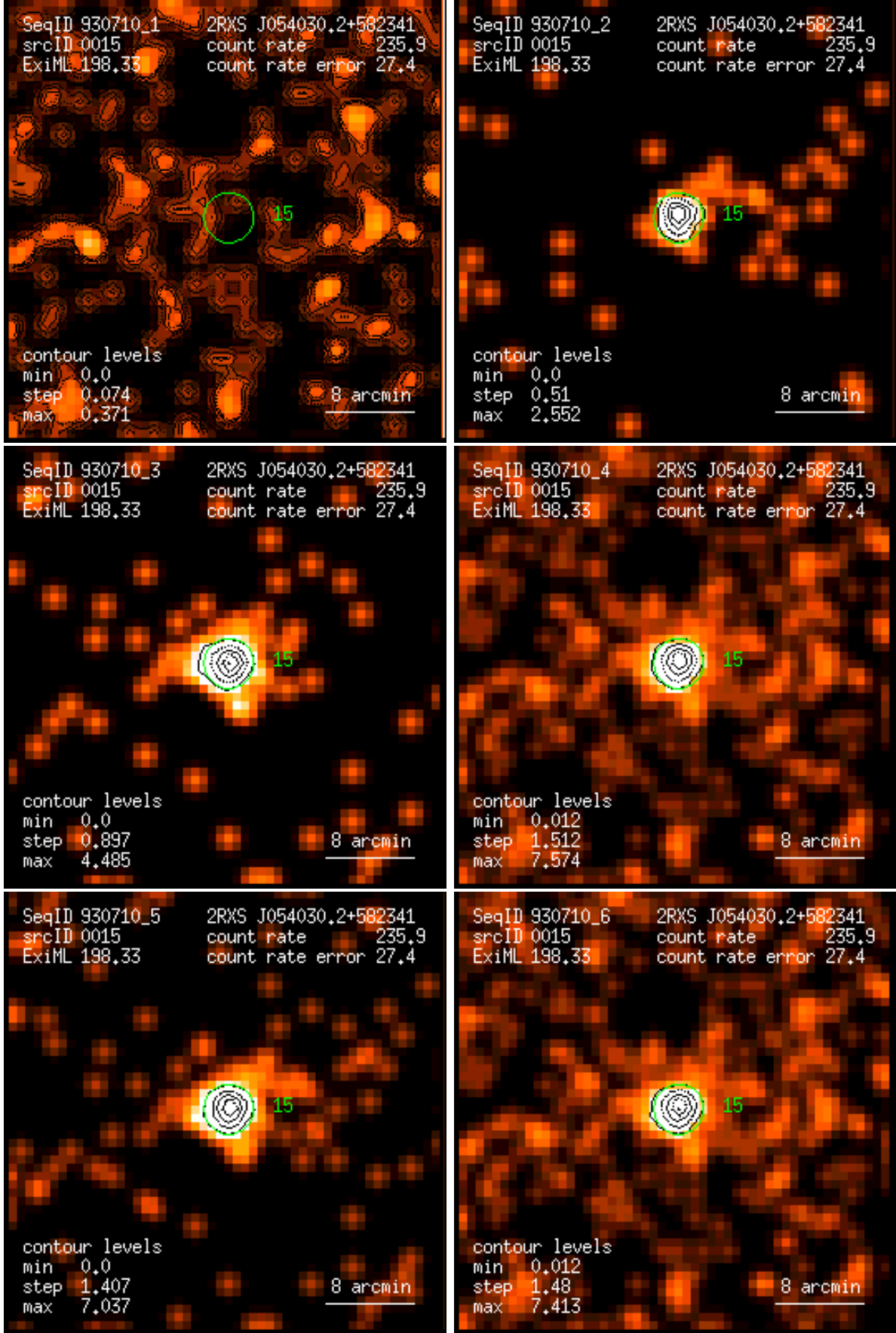
Figure 15: RASS 930710: detection 0015: band rate images, Gaussian filter: (1) PSPC channels 11 – 41, (2) 52 – 90, (3) 91 – 201, (4) 11 – 235, (5) 52 – 201, (6) 11 – 201. Broad band rates in counts/ks. Band rate contour levels in counts/ks/arcmin 2 .
