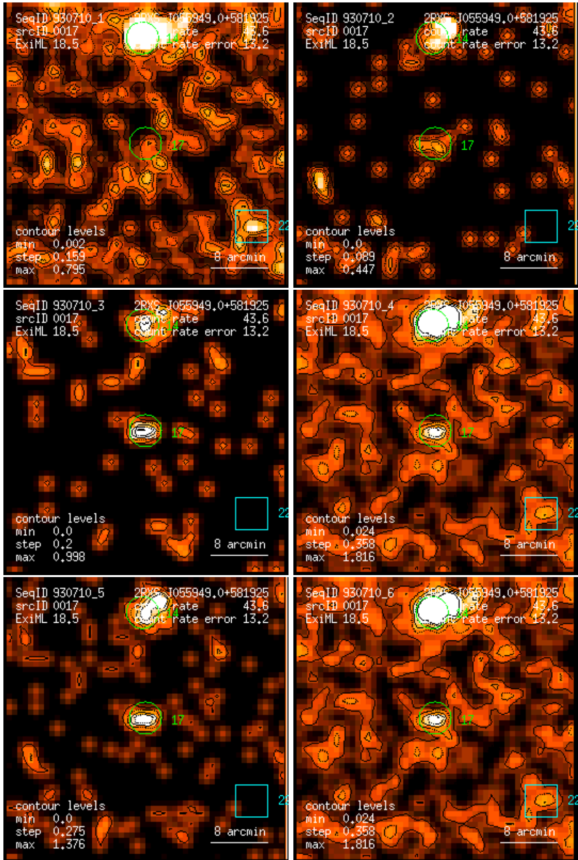
Figure 17: RASS 930710: detection 0017: band rate images, Gaussian filter: (1) PSPC channels 11 – 41, (2) 52 – 90, (3) 91 – 201, (4) 11 – 235, (5) 52 – 201, (6) 11 – 201. Broad band rates in counts/ks. Band rate contour levels in counts/ks/arcmin 2 .
