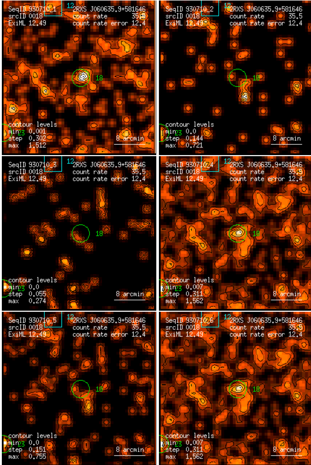
Figure 18: RASS 930710: detection 0018: band rate images, Gaussian filter: (1) PSPC channels 11 – 41, (2) 52 – 90, (3) 91 – 201, (4) 11 – 235, (5) 52 – 201, (6) 11 – 201. Broad band rates in counts/ks. Band rate contour levels in counts/ks/arcmin 2 .
