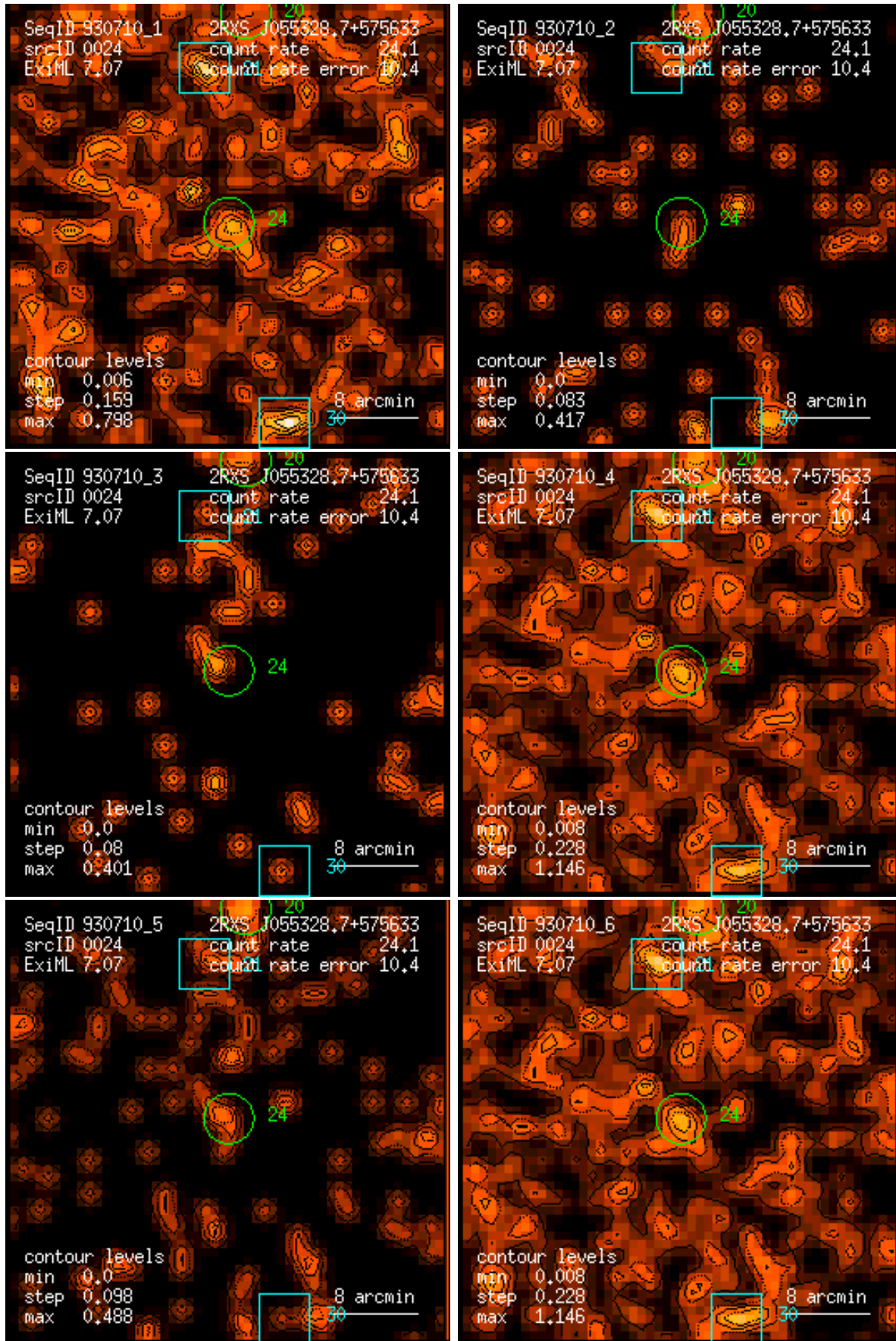
Figure 24: RASS 930710: detection 0024: band rate images, Gaussian filter: (1) PSPC channels 11 – 41, (2) 52 – 90, (3) 91 – 201, (4) 11 – 235, (5) 52 – 201, (6) 11 – 201. Broad band rates in counts/ks. Band rate contour levels in counts/ks/arcmin 2 .
