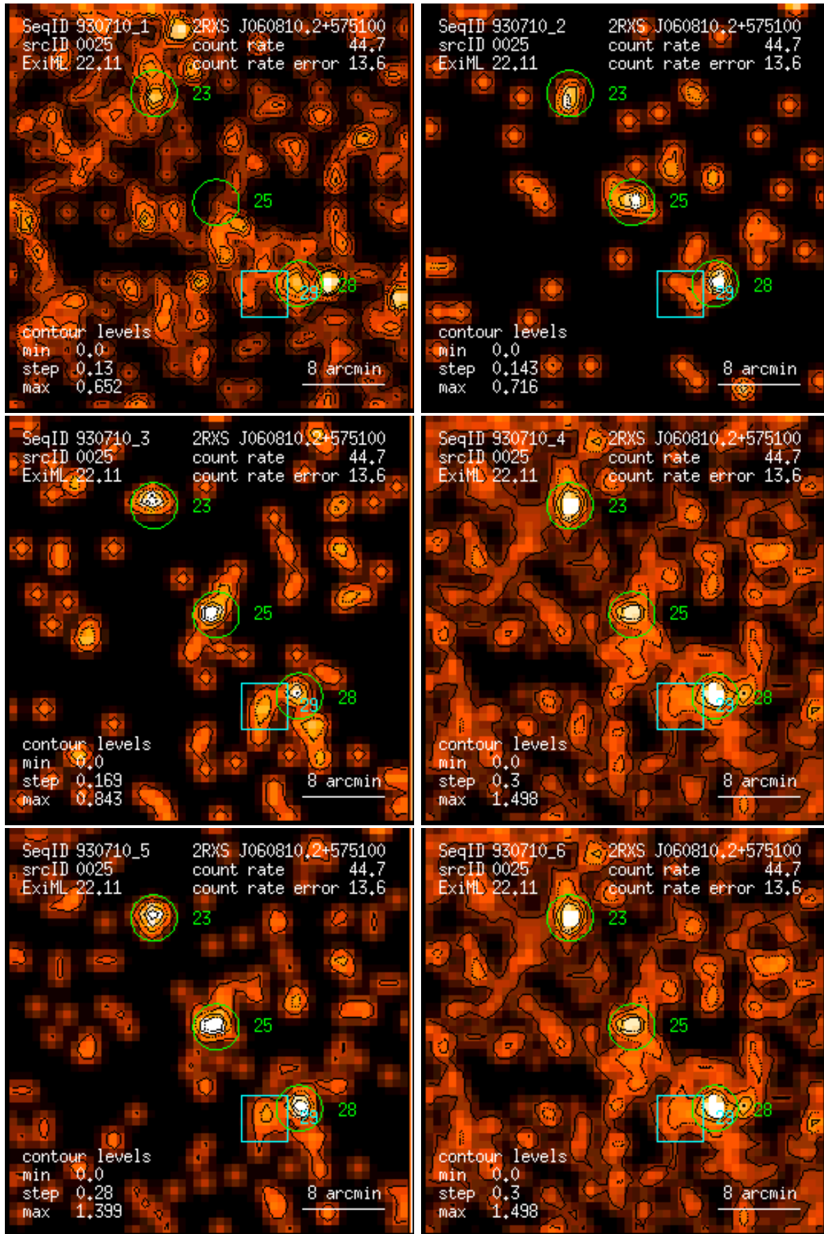
Figure 25: RASS 930710: detection 0025: band rate images, Gaussian filter: (1) PSPC channels 11 – 41, (2) 52 – 90, (3) 91 – 201, (4) 11 – 235, (5) 52 – 201, (6) 11 – 201. Broad band rates in counts/ks. Band rate contour levels in counts/ks/arcmin 2 .
