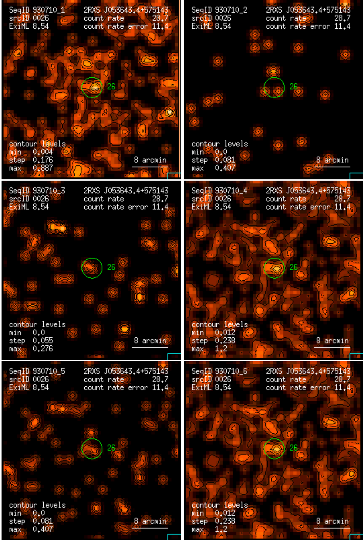
Figure 26: RASS 930710: detection 0026: band rate images, Gaussian filter: (1) PSPC channels 11 – 41, (2) 52 – 90, (3) 91 – 201, (4) 11 – 235, (5) 52 – 201, (6) 11 – 201. Broad band rates in counts/ks. Band rate contour levels in counts/ks/arcmin 2 .
