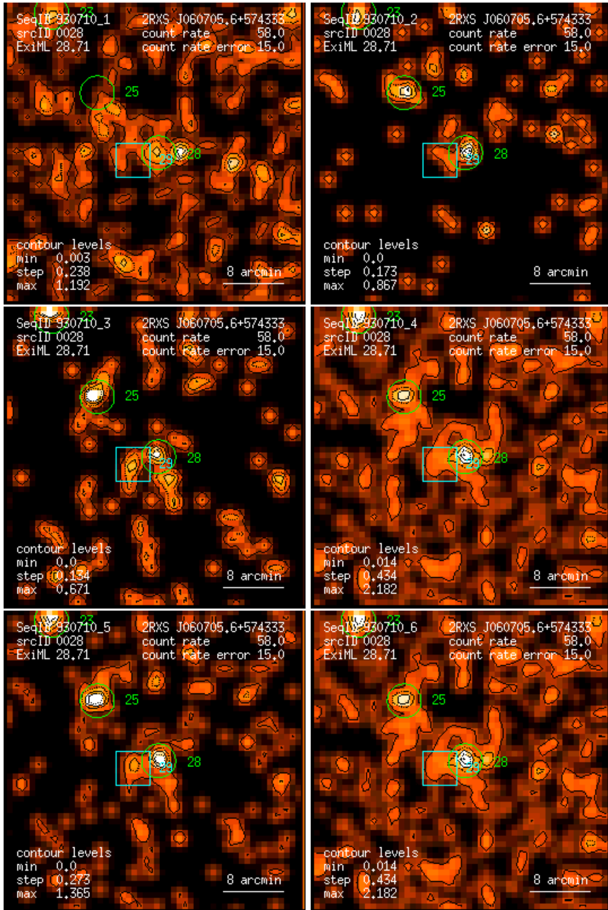
Figure 28: RASS 930710: detection 0028: band rate images, Gaussian filter: (1) PSPC channels 11 – 41, (2) 52 – 90, (3) 91 – 201, (4) 11 – 235, (5) 52 – 201, (6) 11 – 201. Broad band rates in counts/ks. Band rate contour levels in counts/ks/arcmin 2 .
