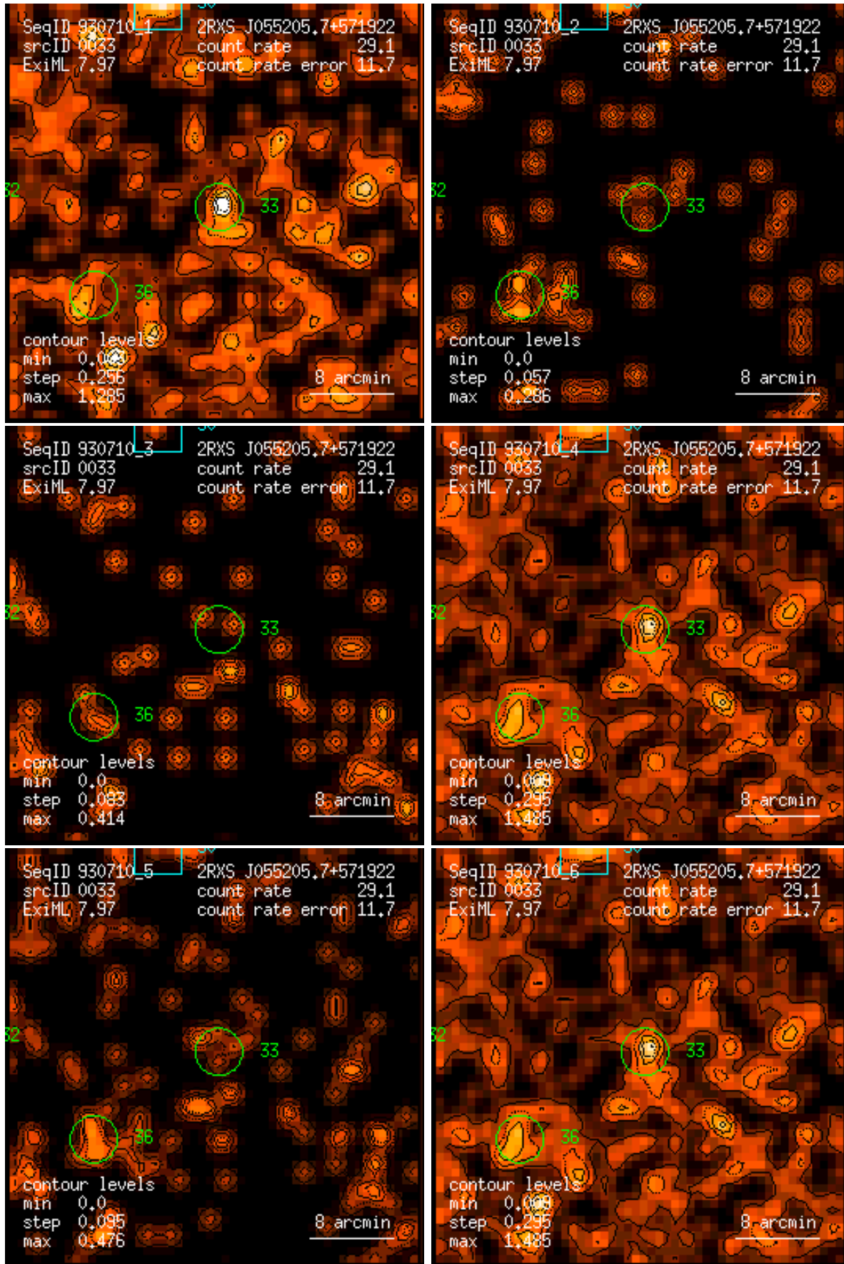
Figure 33: RASS 930710: detection 0033: band rate images, Gaussian filter: (1) PSPC channels 11 – 41, (2) 52 – 90, (3) 91 – 201, (4) 11 – 235, (5) 52 – 201, (6) 11 – 201. Broad band rates in counts/ks. Band rate contour levels in counts/ks/arcmin 2 .
