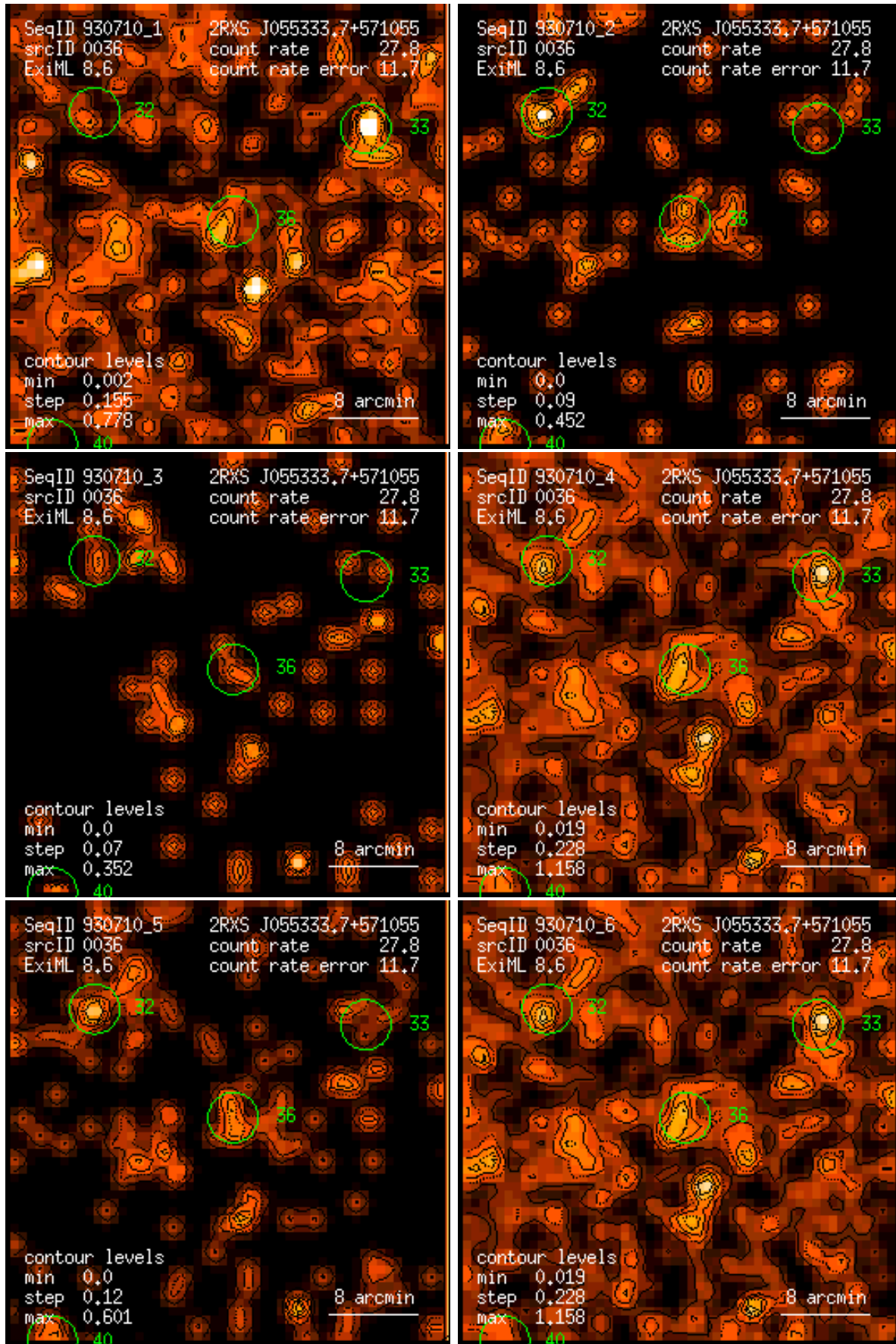
Figure 36: RASS 930710: detection 0036: band rate images, Gaussian filter: (1) PSPC channels 11 – 41, (2) 52 – 90, (3) 91 – 201, (4) 11 – 235, (5) 52 – 201, (6) 11 – 201. Broad band rates in counts/ks. Band rate contour levels in counts/ks/arcmin 2 .
