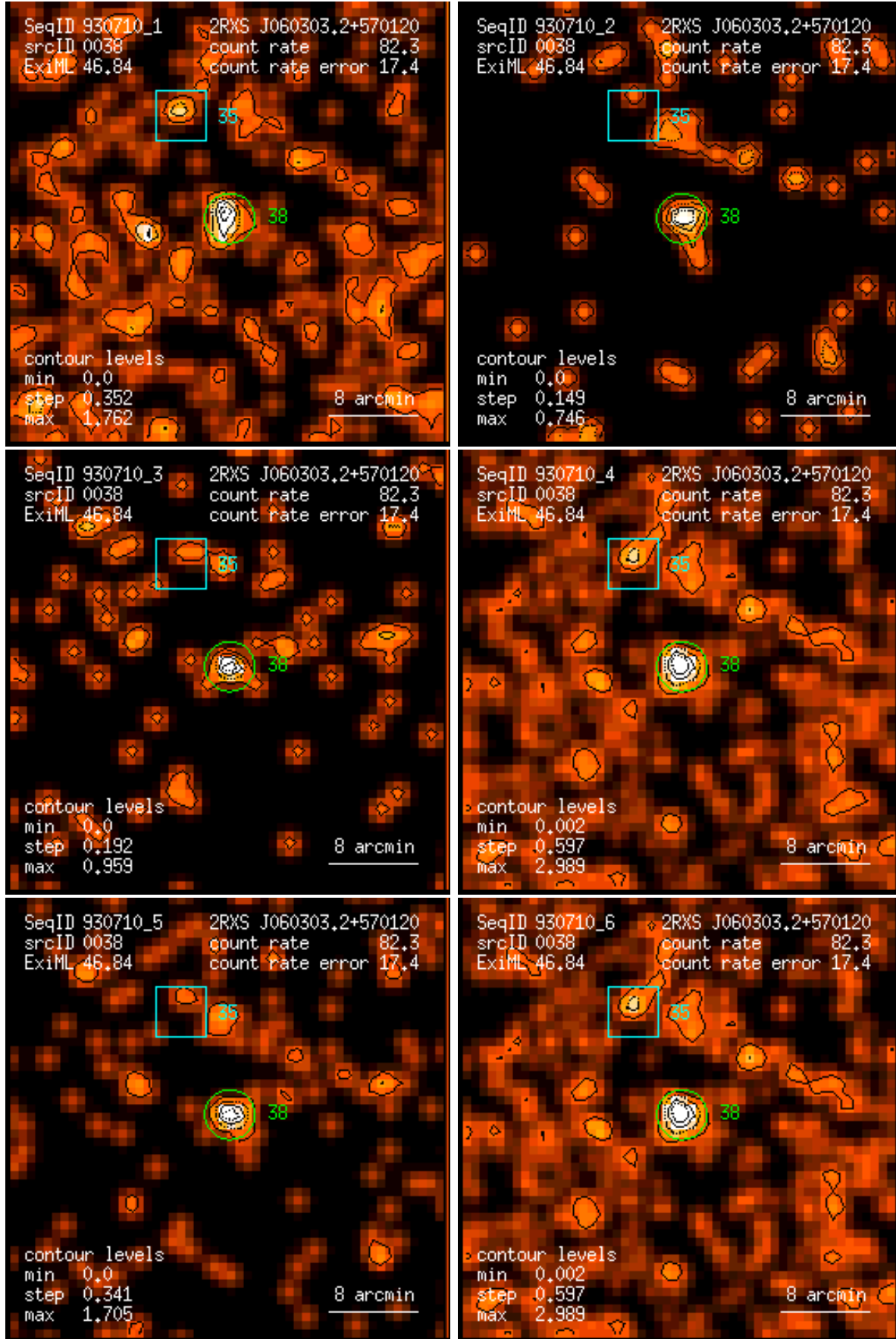
Figure 38: RASS 930710: detection 0038: band rate images, Gaussian filter: (1) PSPC channels 11 – 41, (2) 52 – 90, (3) 91 – 201, (4) 11 – 235, (5) 52 – 201, (6) 11 – 201. Broad band rates in counts/ks. Band rate contour levels in counts/ks/arcmin 2 .
