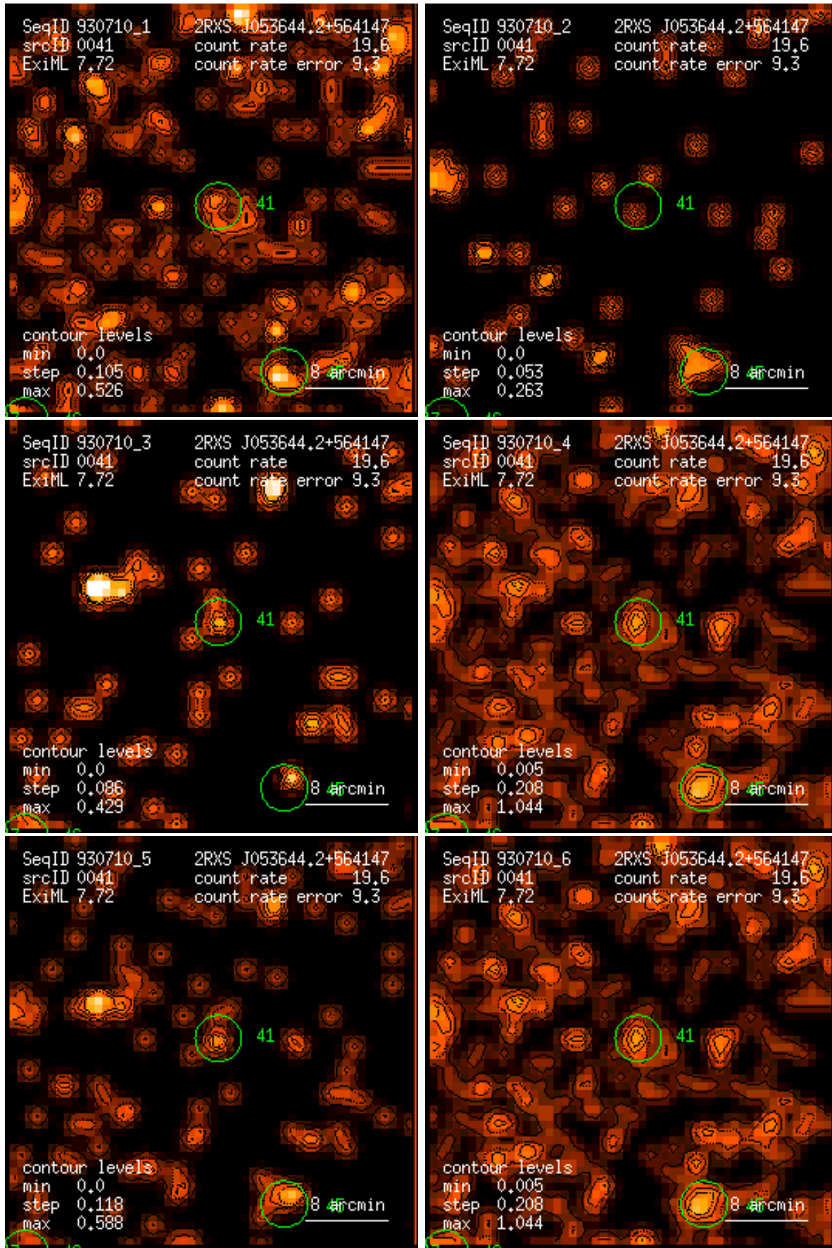
Figure 41: RASS 930710: detection 0041: band rate images, Gaussian filter: (1) PSPC channels 11 – 41, (2) 52 – 90, (3) 91 – 201, (4) 11 – 235, (5) 52 – 201, (6) 11 – 201. Broad band rates in counts/ks. Band rate contour levels in counts/ks/arcmin 2 .
