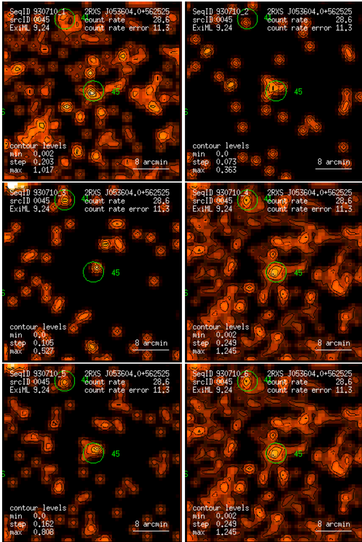
Figure 45: RASS 930710: detection 0045: band rate images, Gaussian filter: (1) PSPC channels 11 – 41, (2) 52 – 90, (3) 91 – 201, (4) 11 – 235, (5) 52 – 201, (6) 11 – 201. Broad band rates in counts/ks. Band rate contour levels in counts/ks/arcmin 2 .
