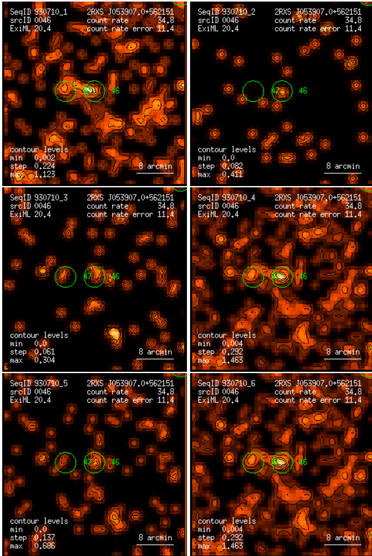
Figure 46: RASS 930710: detection 0046: band rate images, Gaussian filter: (1) PSPC channels 11 – 41, (2) 52 – 90, (3) 91 – 201, (4) 11 – 235, (5) 52 – 201, (6) 11 – 201. Broad band rates in counts/ks. Band rate contour levels in counts/ks/arcmin 2 .
