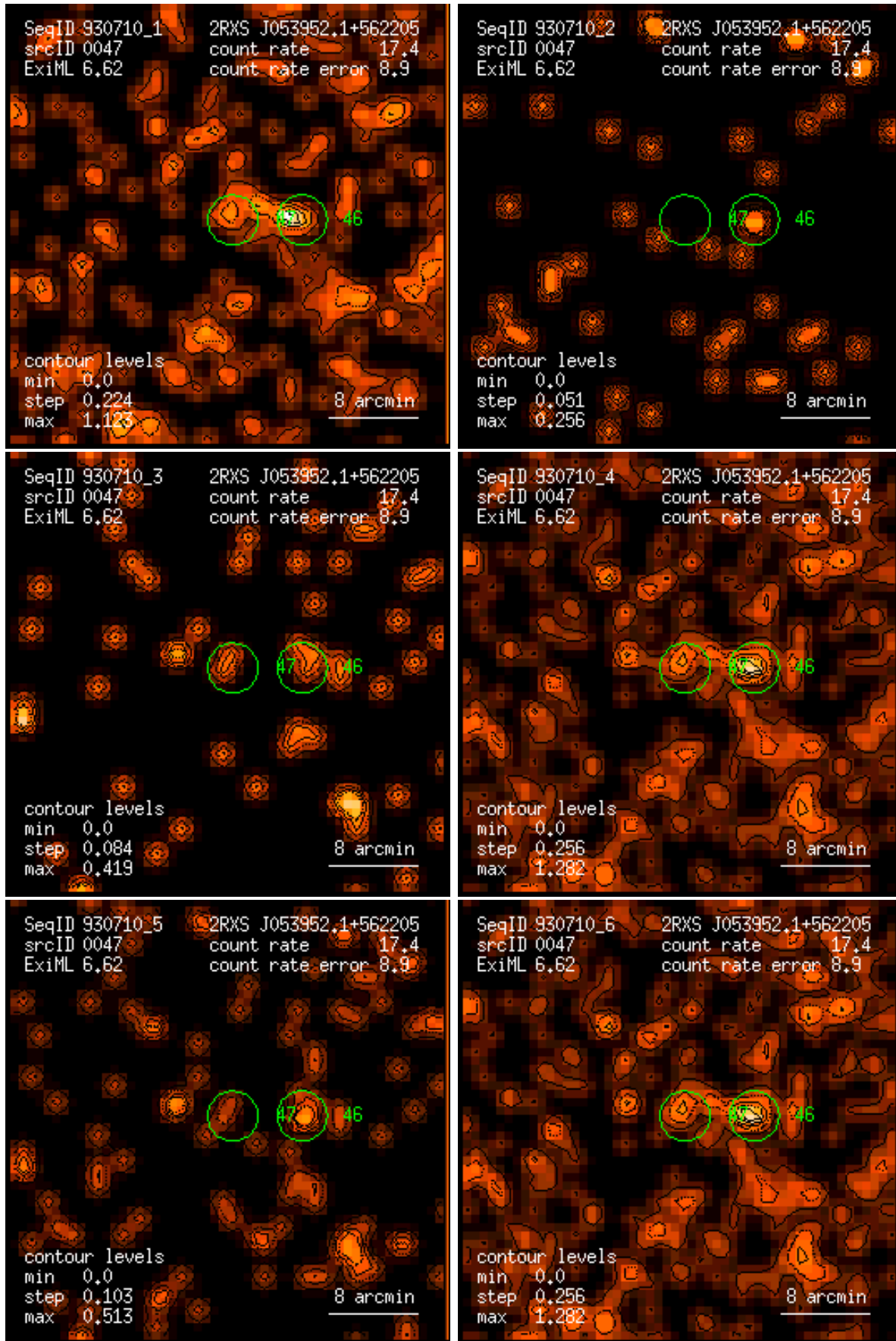
Figure 47: RASS 930710: detection 0047: band rate images, Gaussian filter: (1) PSPC channels 11 – 41, (2) 52 – 90, (3) 91 – 201, (4) 11 – 235, (5) 52 – 201, (6) 11 – 201. Broad band rates in counts/ks. Band rate contour levels in counts/ks/arcmin 2 .
