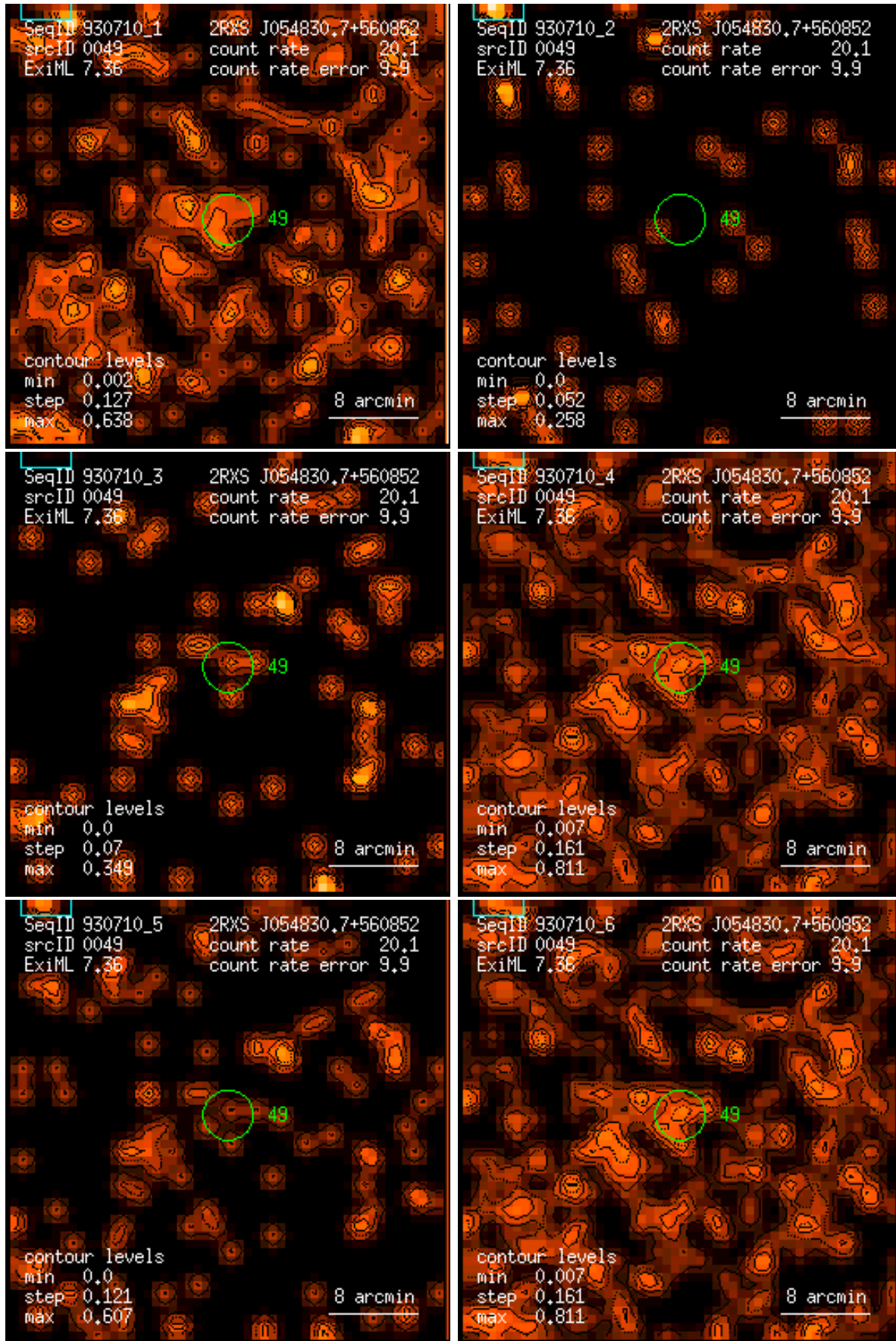
Figure 49: RASS 930710: detection 0049: band rate images, Gaussian filter: (1) PSPC channels 11 – 41, (2) 52 – 90, (3) 91 – 201, (4) 11 – 235, (5) 52 – 201, (6) 11 – 201. Broad band rates in counts/ks. Band rate contour levels in counts/ks/arcmin 2 .
