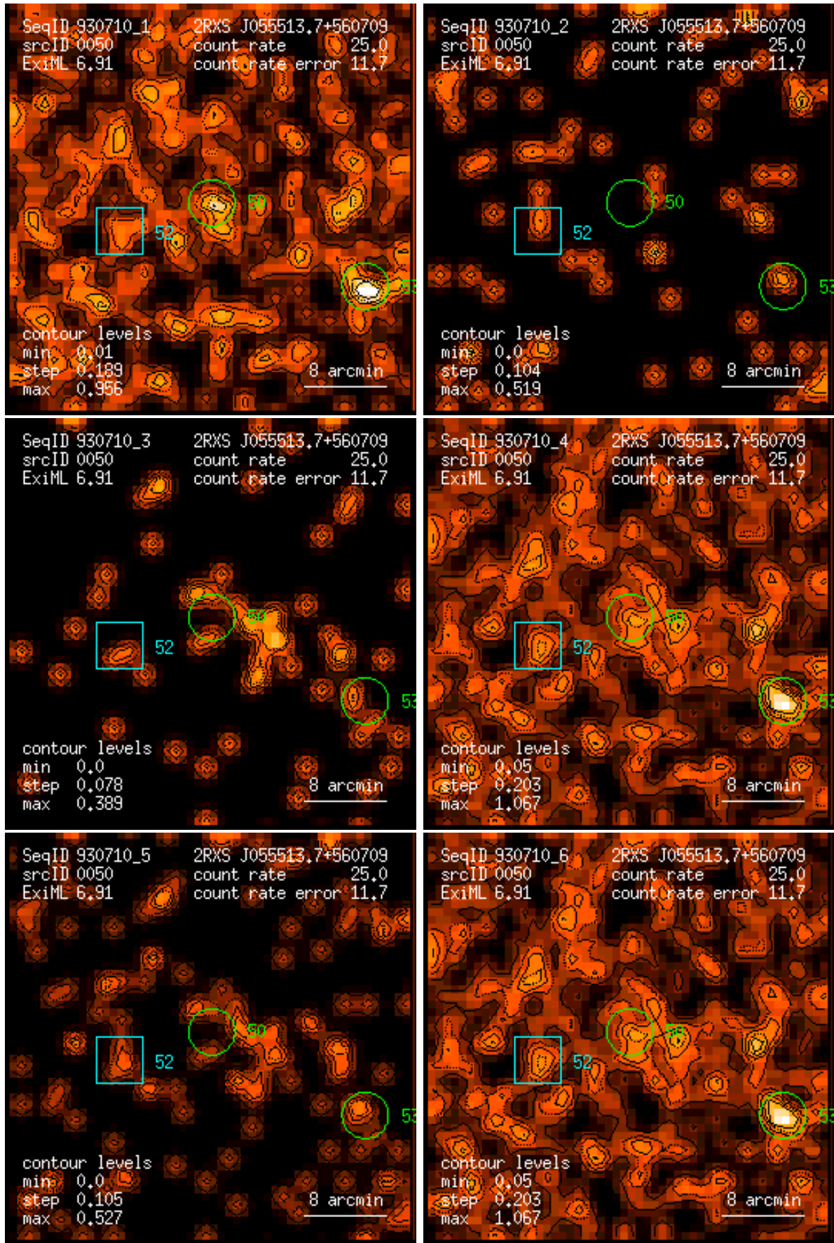
Figure 50: RASS 930710: detection 0050: band rate images, Gaussian filter: (1) PSPC channels 11 – 41, (2) 52 – 90, (3) 91 – 201, (4) 11 – 235, (5) 52 – 201, (6) 11 – 201. Broad band rates in counts/ks. Band rate contour levels in counts/ks/arcmin 2 .
