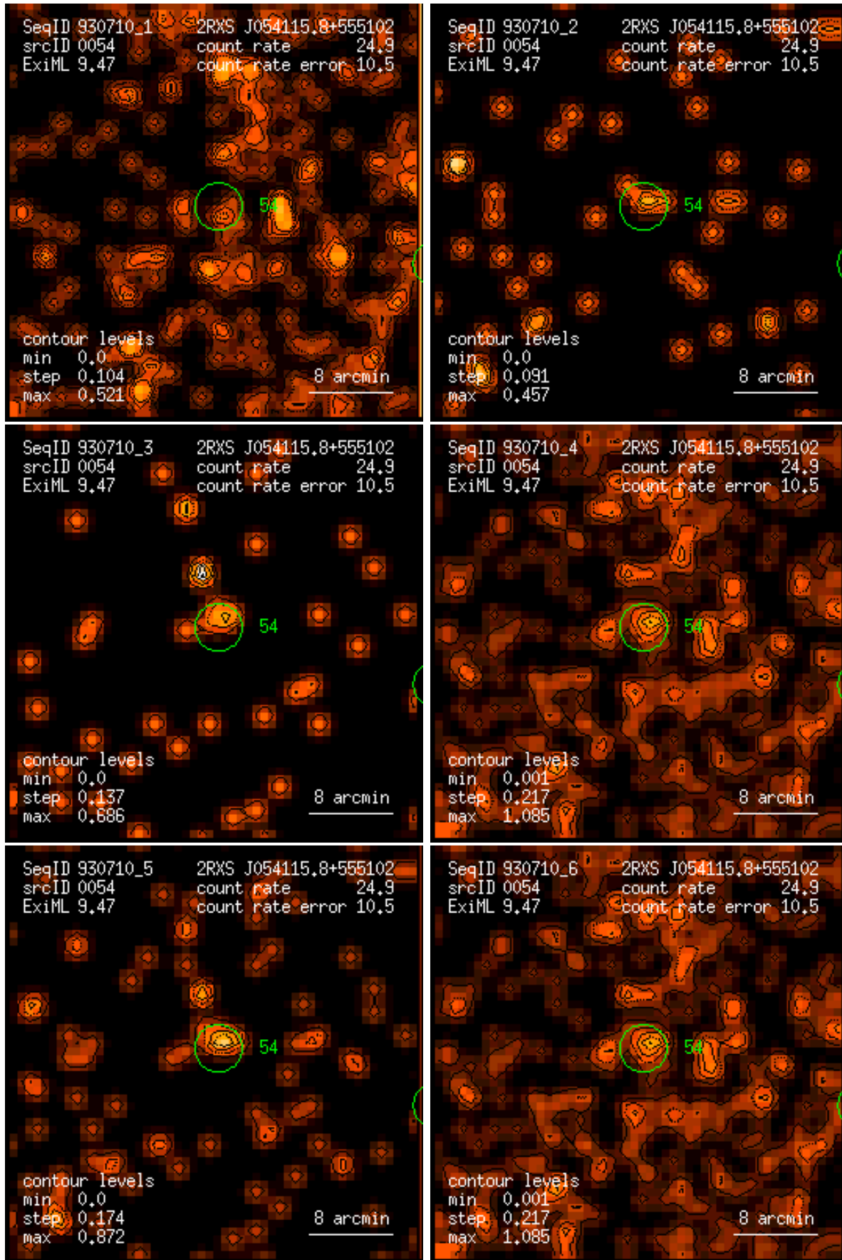
Figure 54: RASS 930710: detection 0054: band rate images, Gaussian filter: (1) PSPC channels 11 – 41, (2) 52 – 90, (3) 91 – 201, (4) 11 – 235, (5) 52 – 201, (6) 11 – 201. Broad band rates in counts/ks. Band rate contour levels in counts/ks/arcmin 2 .
