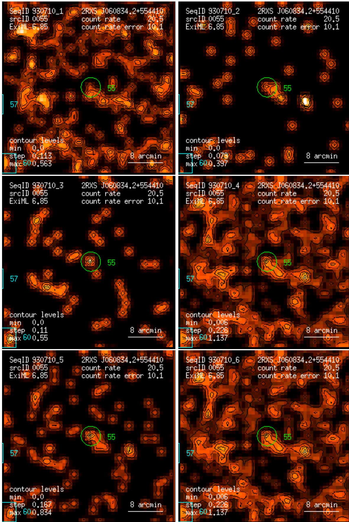
Figure 55: RASS 930710: detection 0055: band rate images, Gaussian filter: (1) PSPC channels 11 – 41, (2) 52 – 90, (3) 91 – 201, (4) 11 – 235, (5) 52 – 201, (6) 11 – 201. Broad band rates in counts/ks. Band rate contour levels in counts/ks/arcmin 2 .
