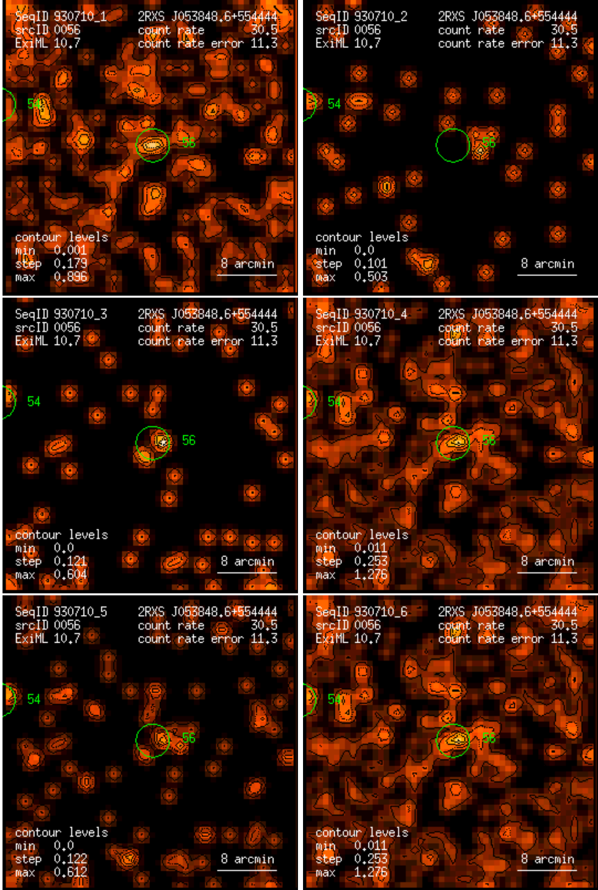
Figure 56: RASS 930710: detection 0056: band rate images, Gaussian filter: (1) PSPC channels 11 – 41, (2) 52 – 90, (3) 91 – 201, (4) 11 – 235, (5) 52 – 201, (6) 11 – 201. Broad band rates in counts/ks. Band rate contour levels in counts/ks/arcmin 2 .
