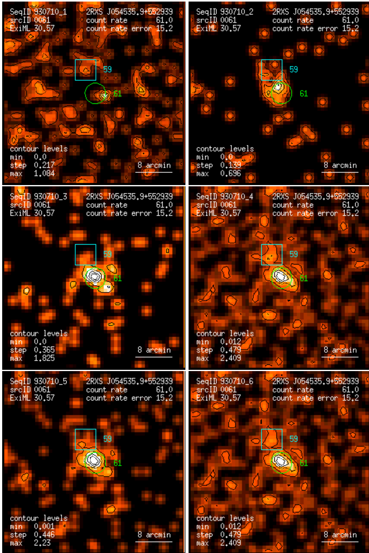
Figure 61: RASS 930710: detection 0061: band rate images, Gaussian filter: (1) PSPC channels 11 – 41, (2) 52 – 90, (3) 91 – 201, (4) 11 – 235, (5) 52 – 201, (6) 11 – 201. Broad band rates in counts/ks. Band rate contour levels in counts/ks/arcmin 2 .
