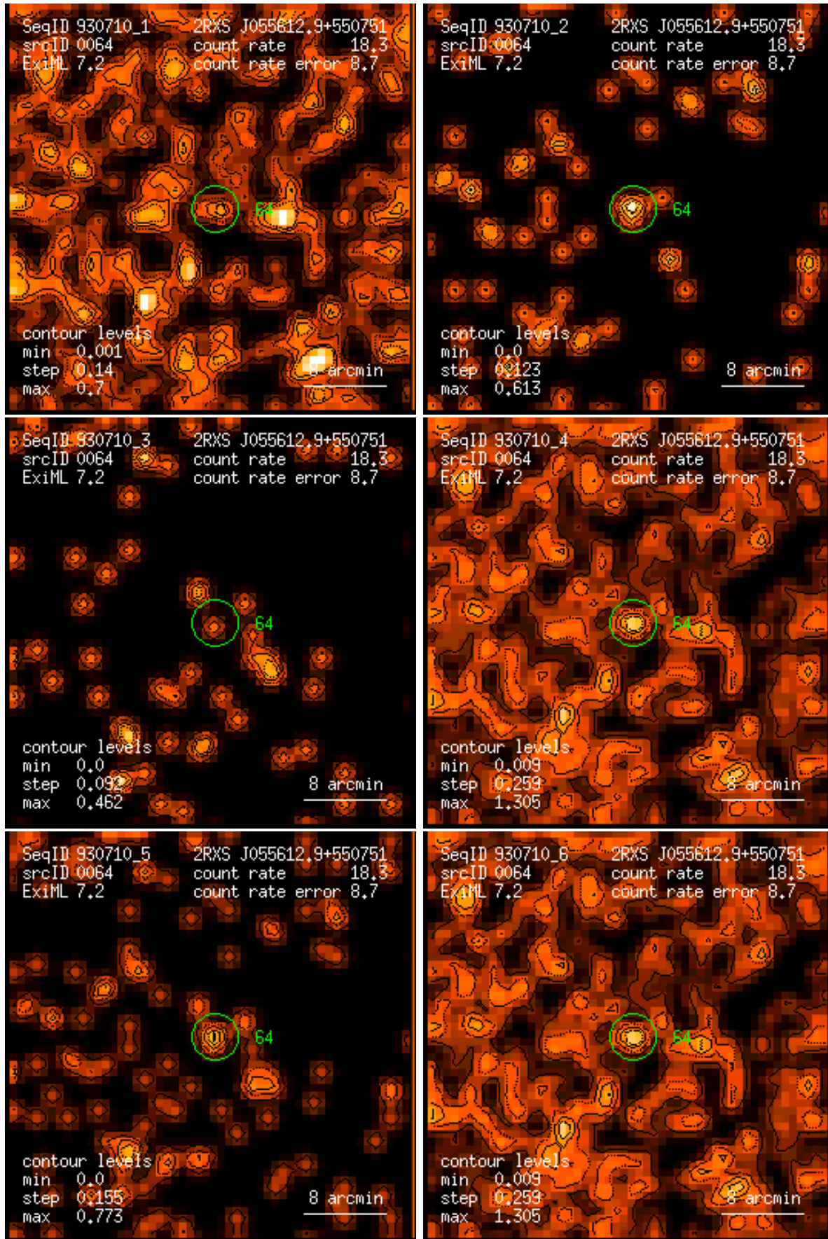
Figure 64: RASS 930710: detection 0064: band rate images, Gaussian filter: (1) PSPC channels 11 – 41, (2) 52 – 90, (3) 91 – 201, (4) 11 – 235, (5) 52 – 201, (6) 11 – 201. Broad band rates in counts/ks. Band rate contour levels in counts/ks/arcmin 2 .
