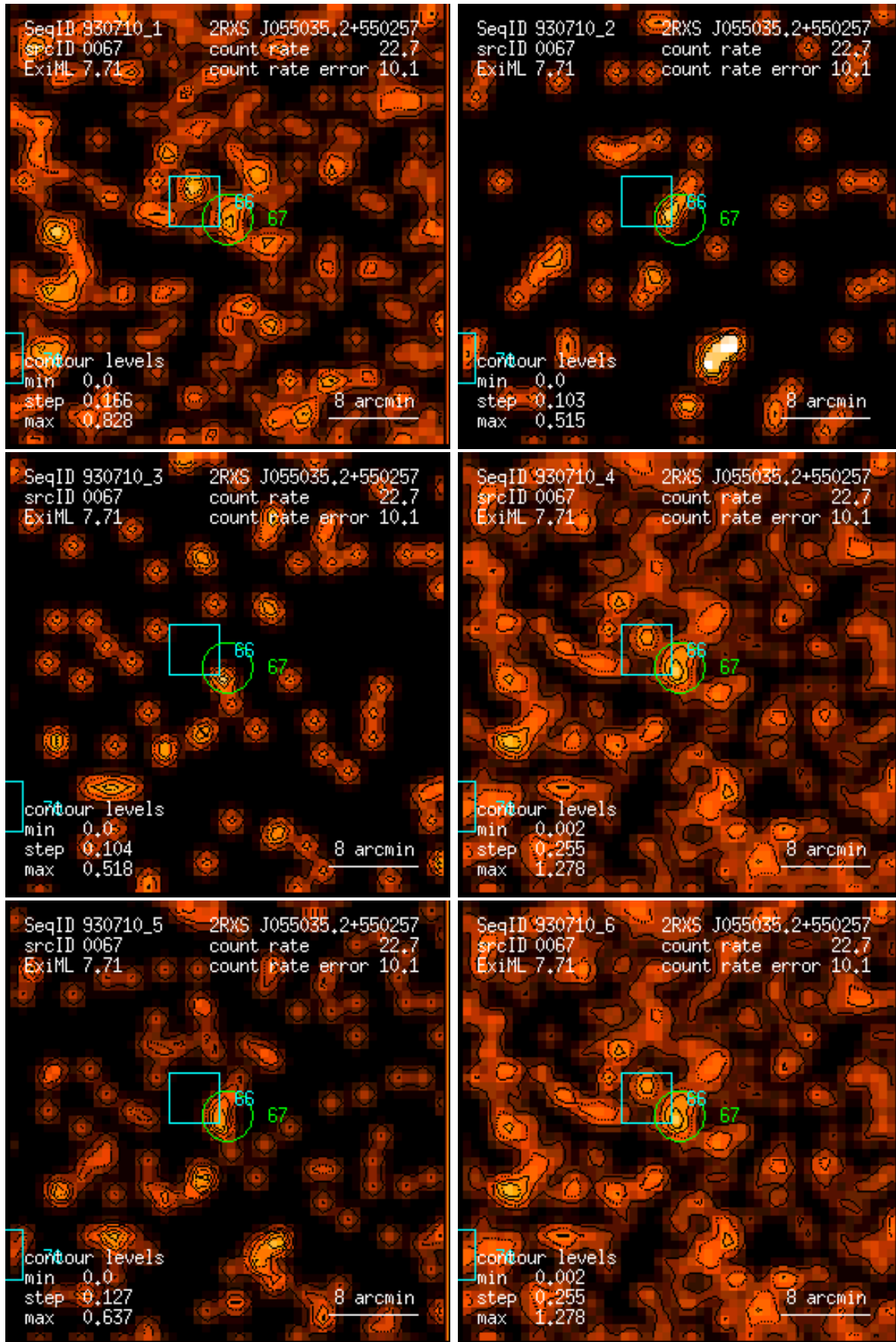
Figure 67: RASS 930710: detection 0067: band rate images, Gaussian filter: (1) PSPC channels 11 – 41, (2) 52 – 90, (3) 91 – 201, (4) 11 – 235, (5) 52 – 201, (6) 11 – 201. Broad band rates in counts/ks. Band rate contour levels in counts/ks/arcmin 2 .
