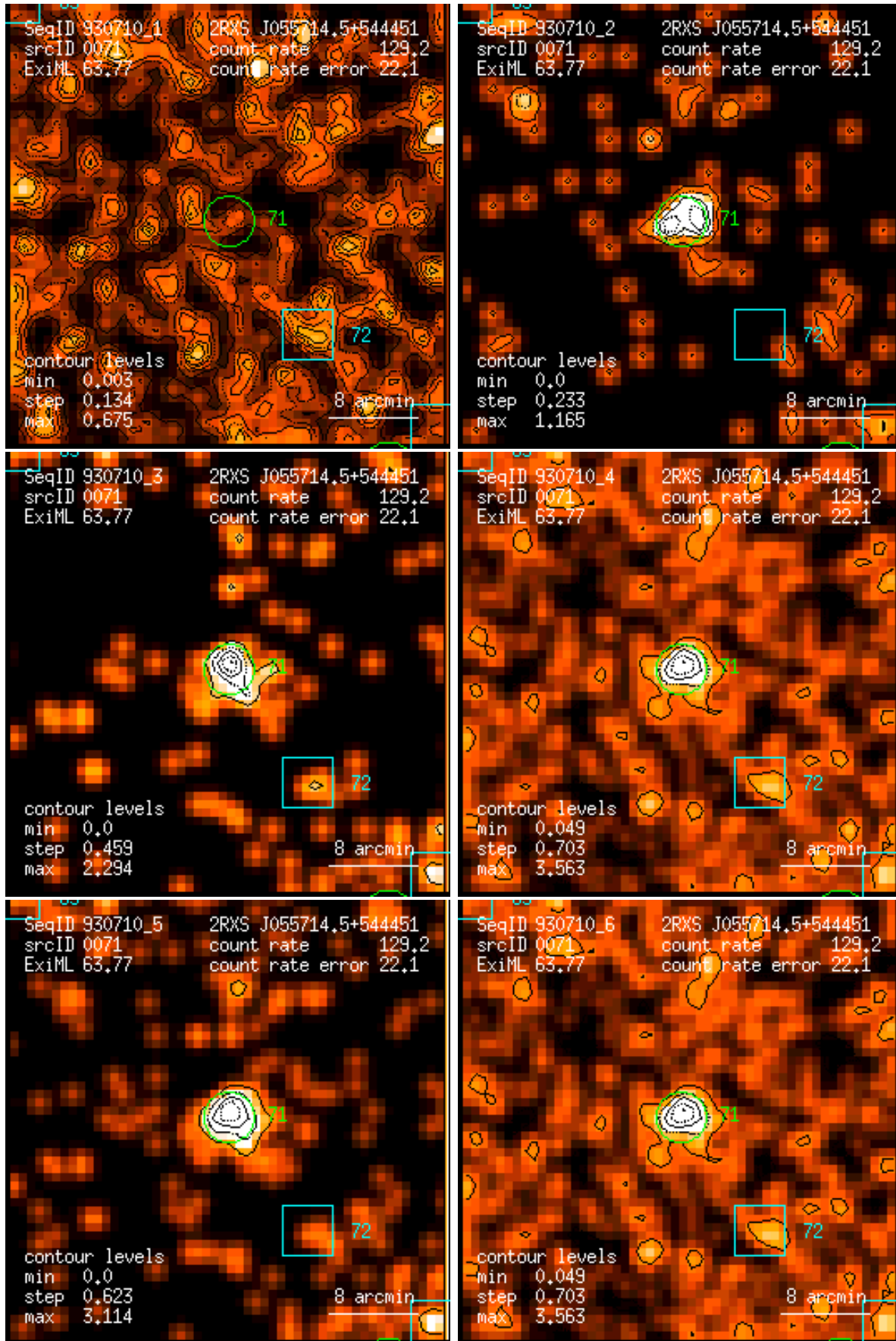
Figure 71: RASS 930710: detection 0071: band rate images, Gaussian filter: (1) PSPC channels 11 – 41, (2) 52 – 90, (3) 91 – 201, (4) 11 – 235, (5) 52 – 201, (6) 11 – 201. Broad band rates in counts/ks. Band rate contour levels in counts/ks/arcmin 2 .
