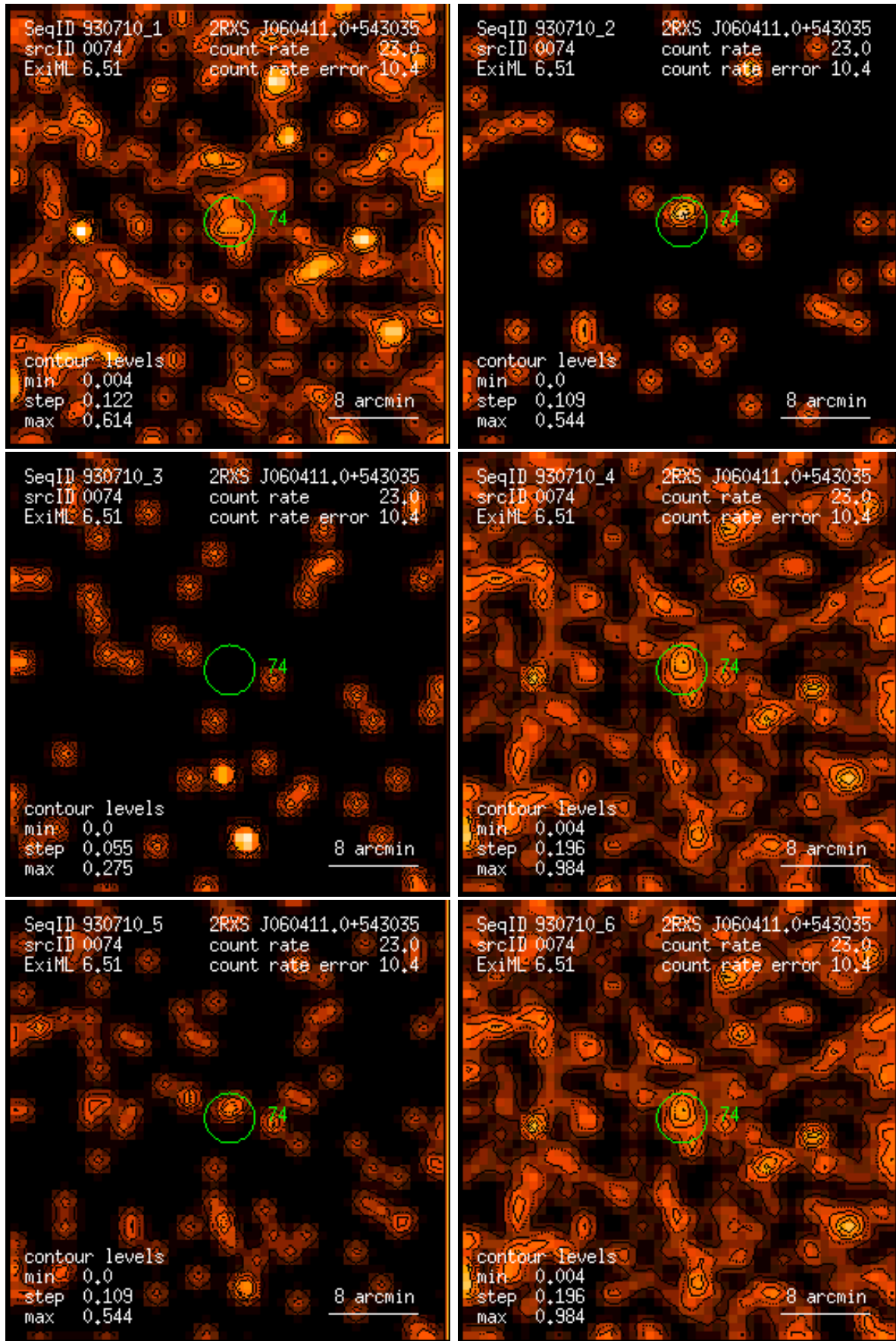
Figure 74: RASS 930710: detection 0074: band rate images, Gaussian filter: (1) PSPC channels 11 – 41, (2) 52 – 90, (3) 91 – 201, (4) 11 – 235, (5) 52 – 201, (6) 11 – 201. Broad band rates in counts/ks. Band rate contour levels in counts/ks/arcmin 2 .
