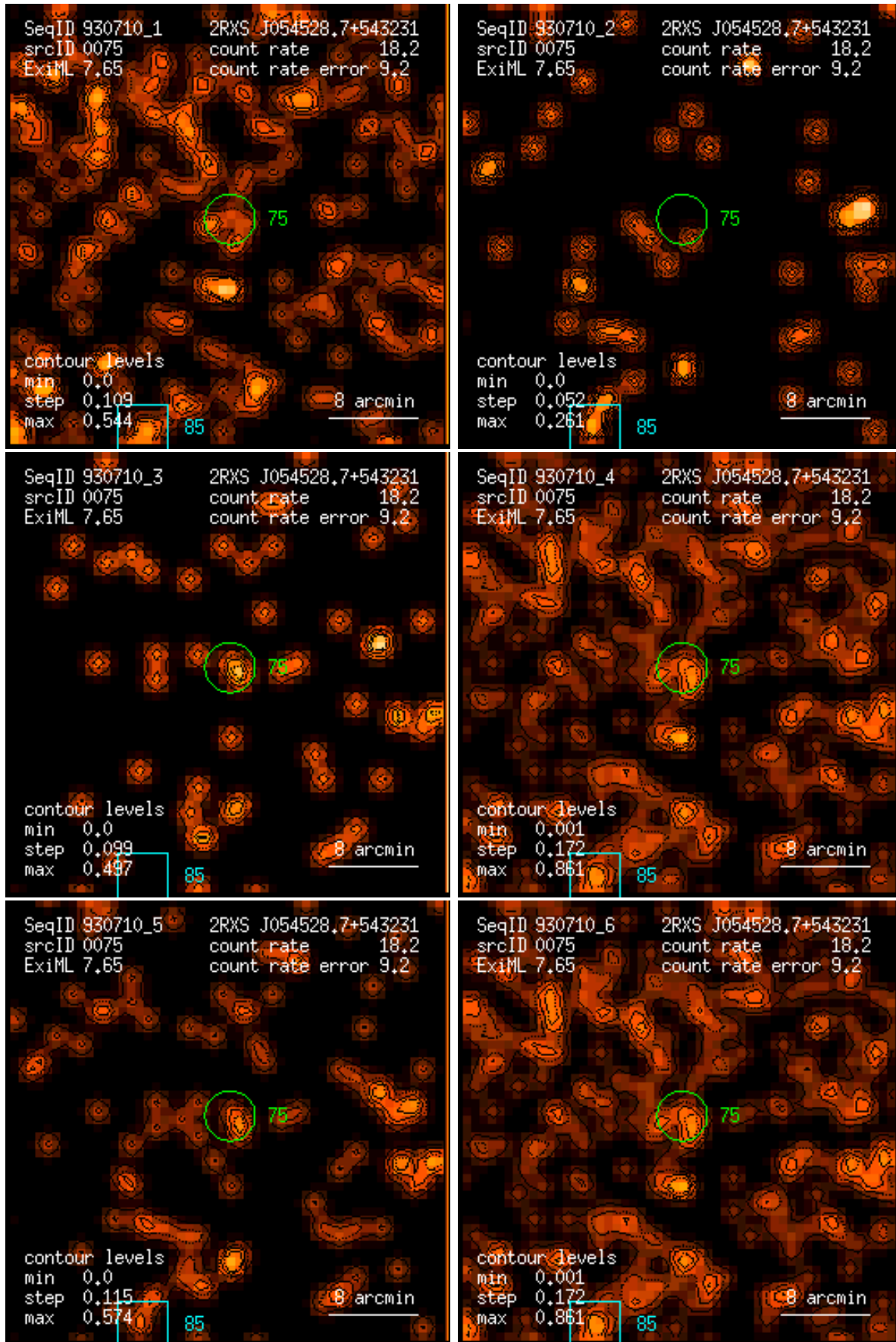
Figure 75: RASS 930710: detection 0075: band rate images, Gaussian filter: (1) PSPC channels 11 – 41, (2) 52 – 90, (3) 91 – 201, (4) 11 – 235, (5) 52 – 201, (6) 11 – 201. Broad band rates in counts/ks. Band rate contour levels in counts/ks/arcmin 2 .
