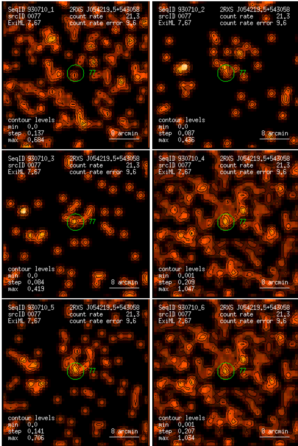
Figure 77: RASS 930710: detection 0077: band rate images, Gaussian filter: (1) PSPC channels 11 – 41, (2) 52 – 90, (3) 91 – 201, (4) 11 – 235, (5) 52 – 201, (6) 11 – 201. Broad band rates in counts/ks. Band rate contour levels in counts/ks/arcmin 2 .
