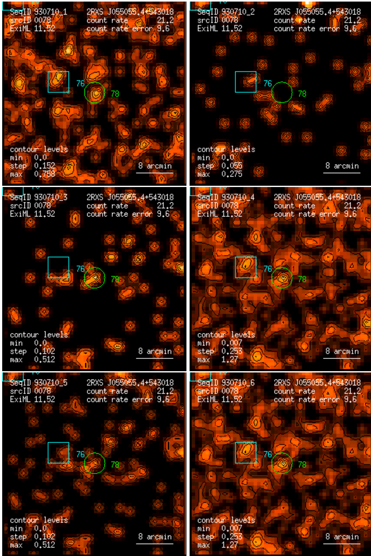
Figure 78: RASS 930710: detection 0078: band rate images, Gaussian filter: (1) PSPC channels 11 – 41, (2) 52 – 90, (3) 91 – 201, (4) 11 – 235, (5) 52 – 201, (6) 11 – 201. Broad band rates in counts/ks. Band rate contour levels in counts/ks/arcmin 2 .
