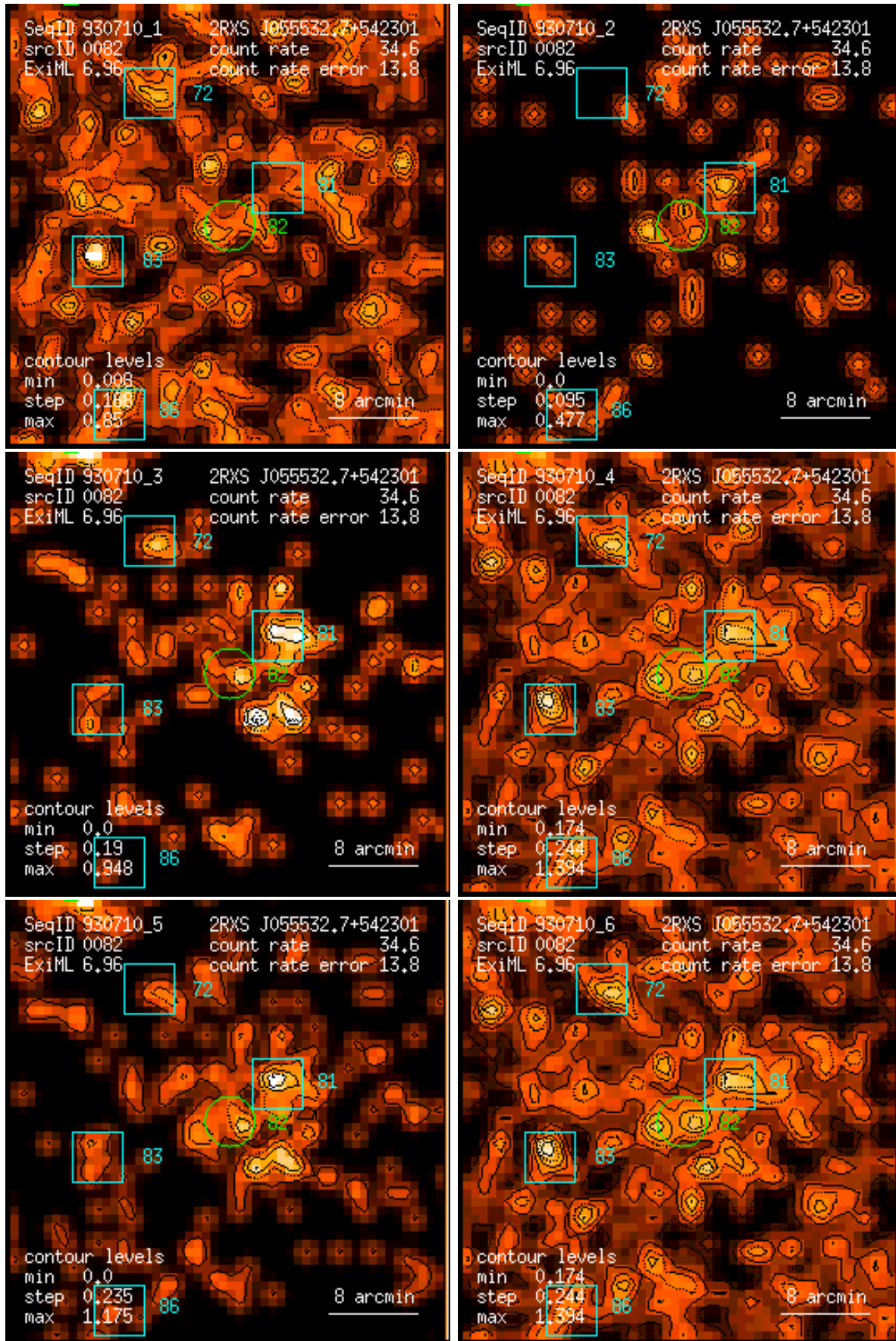
Figure 82: RASS 930710: detection 0082: band rate images, Gaussian filter: (1) PSPC channels 11 – 41, (2) 52 – 90, (3) 91 – 201, (4) 11 – 235, (5) 52 – 201, (6) 11 – 201. Broad band rates in counts/ks. Band rate contour levels in counts/ks/arcmin 2 .
