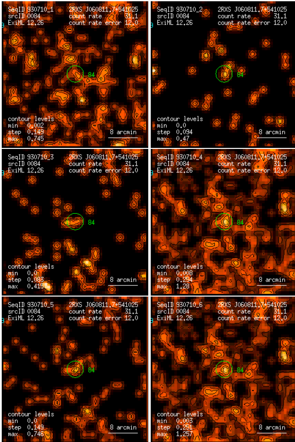
Figure 84: RASS 930710: detection 0084: band rate images, Gaussian filter: (1) PSPC channels 11 – 41, (2) 52 – 90, (3) 91 – 201, (4) 11 – 235, (5) 52 – 201, (6) 11 – 201. Broad band rates in counts/ks. Band rate contour levels in counts/ks/arcmin 2 .
