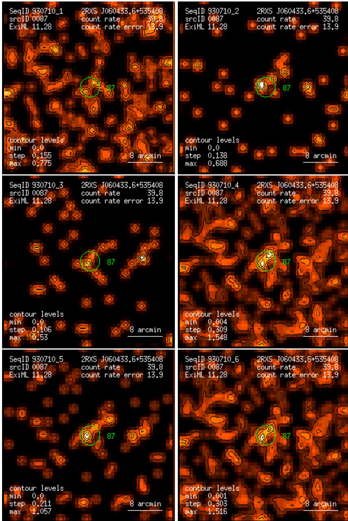
Figure 87: RASS 930710: detection 0087: band rate images, Gaussian filter: (1) PSPC channels 11 – 41, (2) 52 – 90, (3) 91 – 201, (4) 11 – 235, (5) 52 – 201, (6) 11 – 201. Broad band rates in counts/ks. Band rate contour levels in counts/ks/arcmin 2 .
