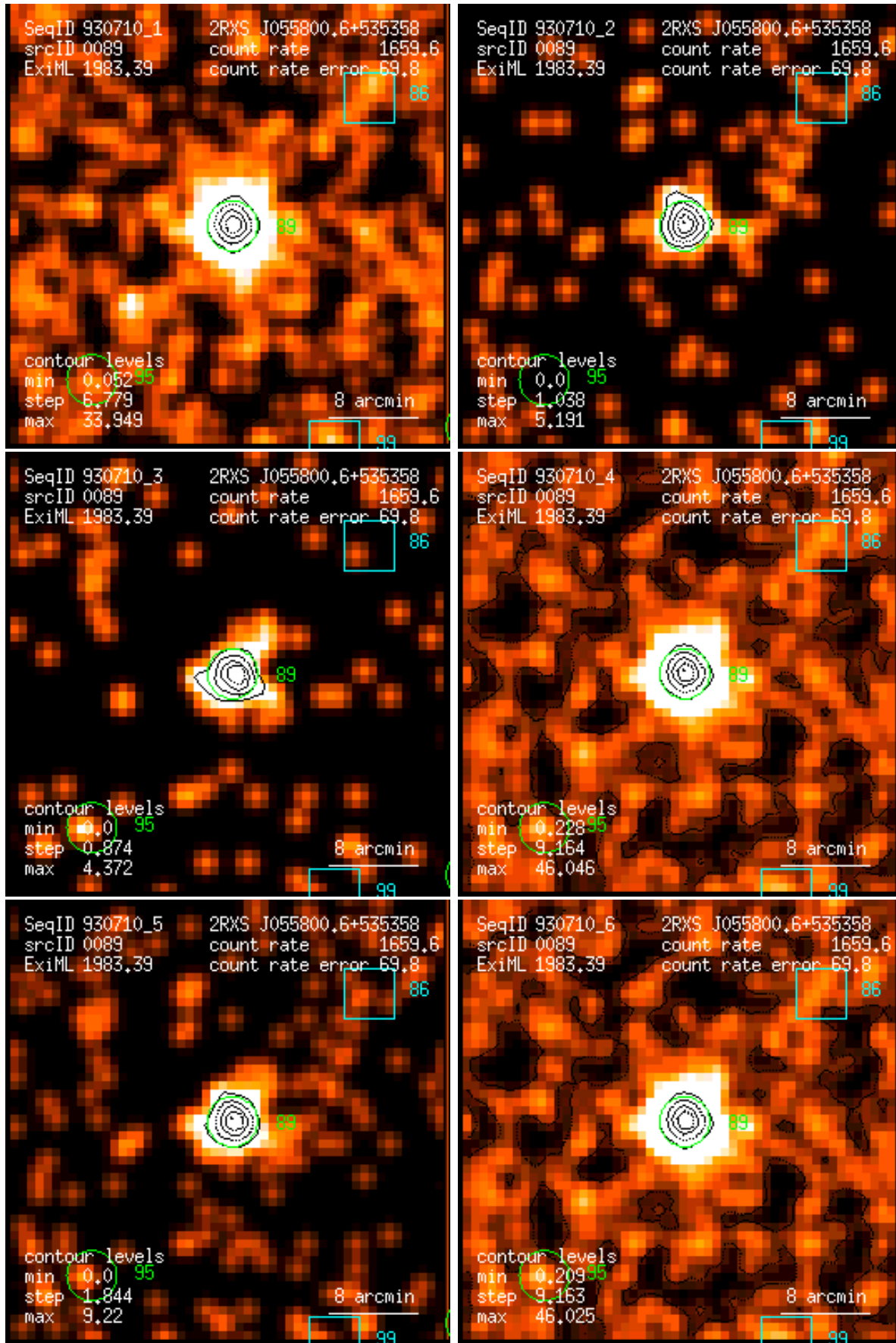
Figure 89: RASS 930710: detection 0089: band rate images, Gaussian filter: (1) PSPC channels 11 – 41, (2) 52 – 90, (3) 91 – 201, (4) 11 – 235, (5) 52 – 201, (6) 11 – 201. Broad band rates in counts/ks. Band rate contour levels in counts/ks/arcmin 2 .
