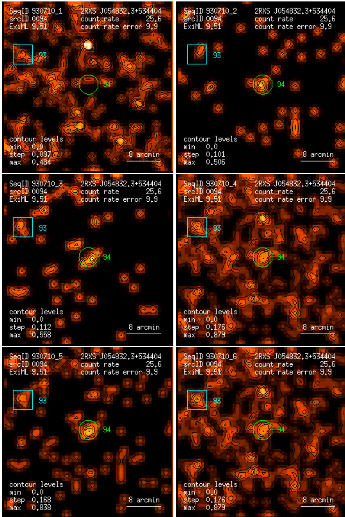
Figure 94: RASS 930710: detection 0094: band rate images, Gaussian filter: (1) PSPC channels 11 – 41, (2) 52 – 90, (3) 91 – 201, (4) 11 – 235, (5) 52 – 201, (6) 11 – 201. Broad band rates in counts/ks. Band rate contour levels in counts/ks/arcmin 2 .
