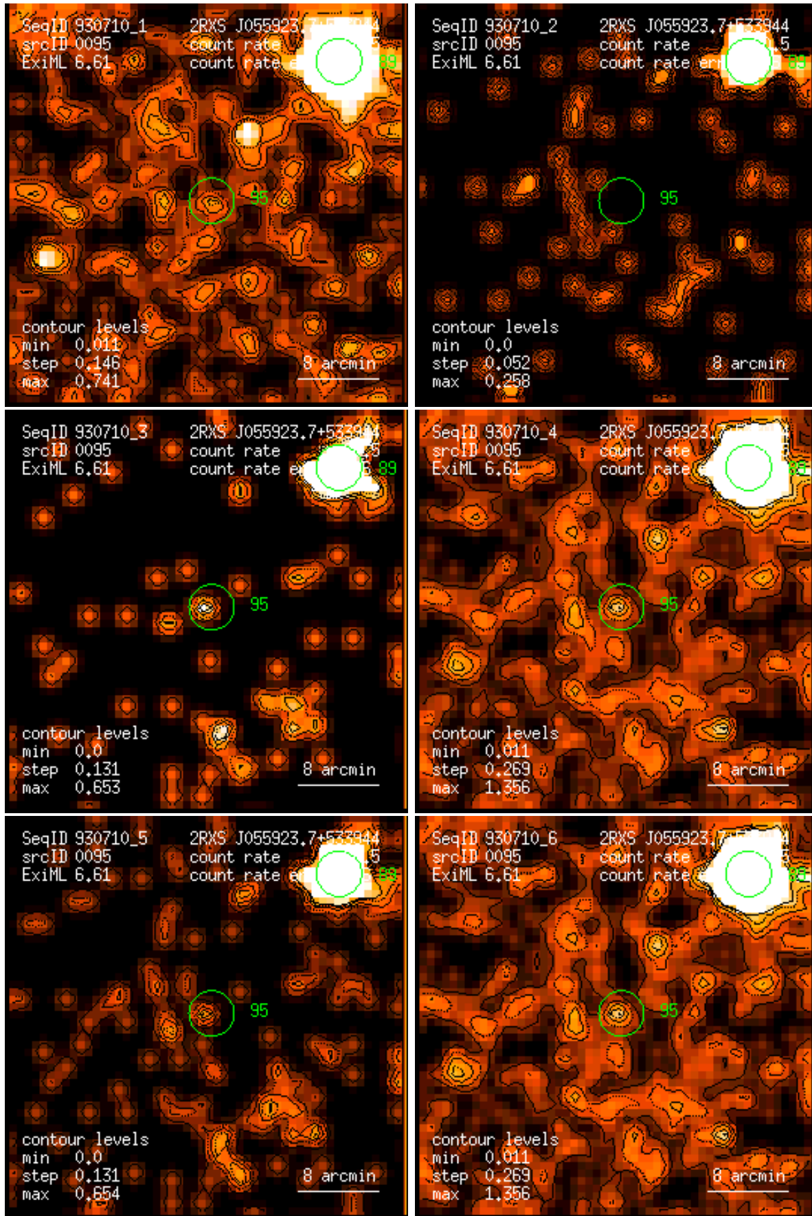
Figure 95: RASS 930710: detection 0095: band rate images, Gaussian filter: (1) PSPC channels 11 – 41, (2) 52 – 90, (3) 91 – 201, (4) 11 – 235, (5) 52 – 201, (6) 11 – 201. Broad band rates in counts/ks. Band rate contour levels in counts/ks/arcmin 2 .
