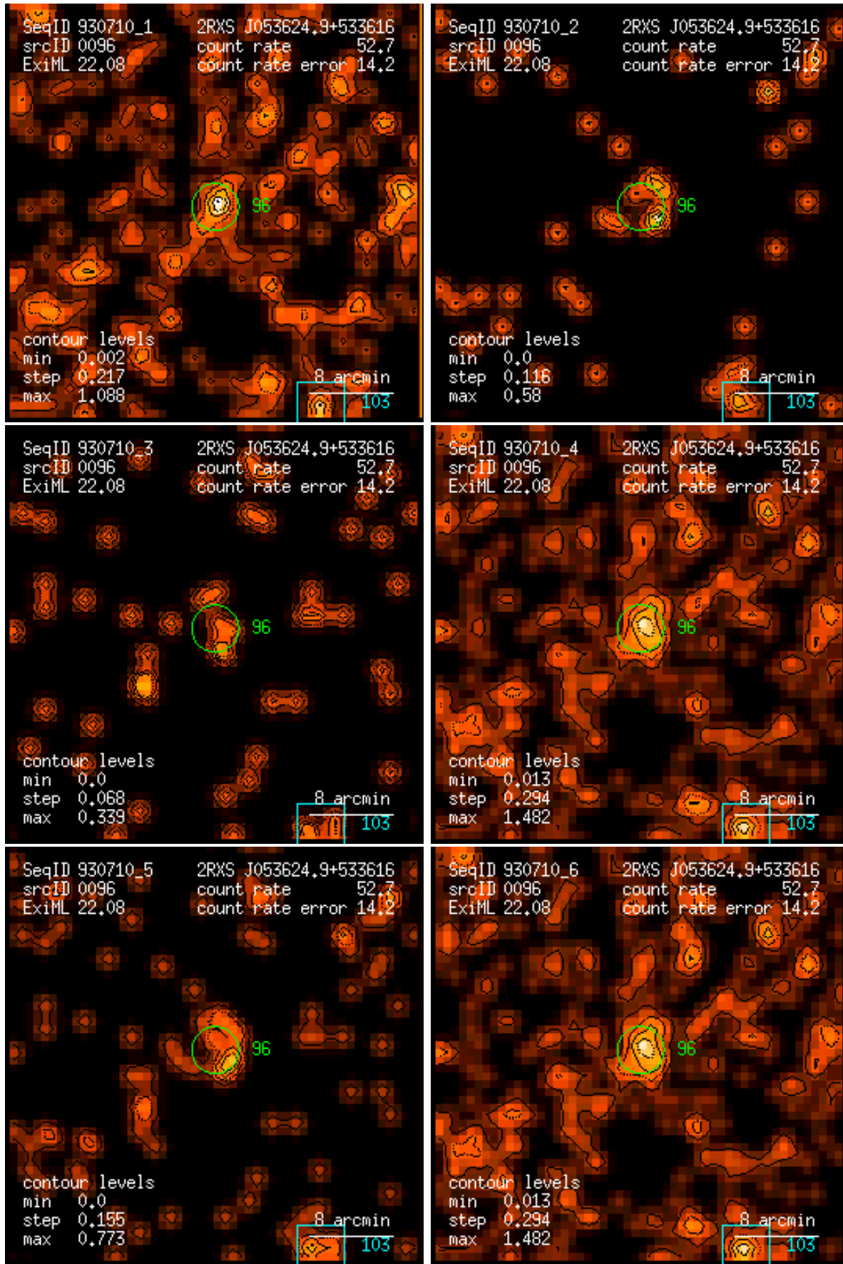
Figure 96: RASS 930710: detection 0096: band rate images, Gaussian filter: (1) PSPC channels 11 – 41, (2) 52 – 90, (3) 91 – 201, (4) 11 – 235, (5) 52 – 201, (6) 11 – 201. Broad band rates in counts/ks. Band rate contour levels in counts/ks/arcmin 2 .
