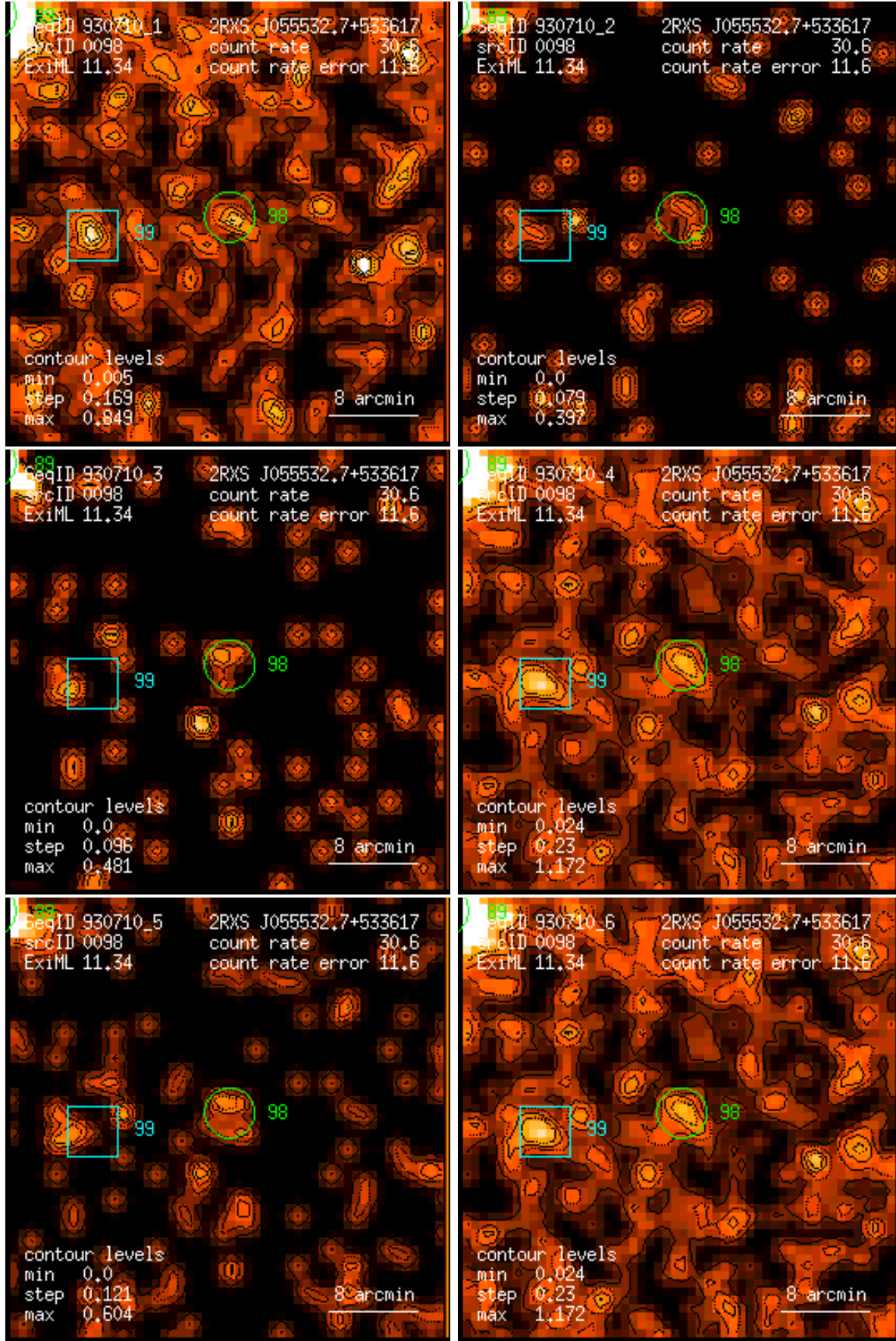
Figure 98: RASS 930710: detection 0098: band rate images, Gaussian filter: (1) PSPC channels 11 – 41, (2) 52 – 90, (3) 91 – 201, (4) 11 – 235, (5) 52 – 201, (6) 11 – 201. Broad band rates in counts/ks. Band rate contour levels in counts/ks/arcmin 2 .
