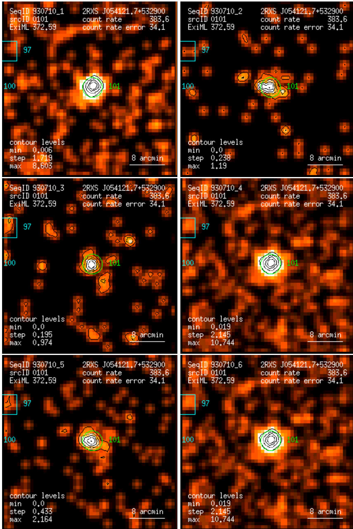
Figure 101: RASS 930710: detection 0101: band rate images, Gaussian filter: (1) PSPC channels 11 – 41, (2) 52 – 90, (3) 91 – 201, (4) 11 – 235, (5) 52 – 201, (6) 11 – 201. Broad band rates in counts/ks. Band rate contour levels in counts/ks/arcmin 2 .
