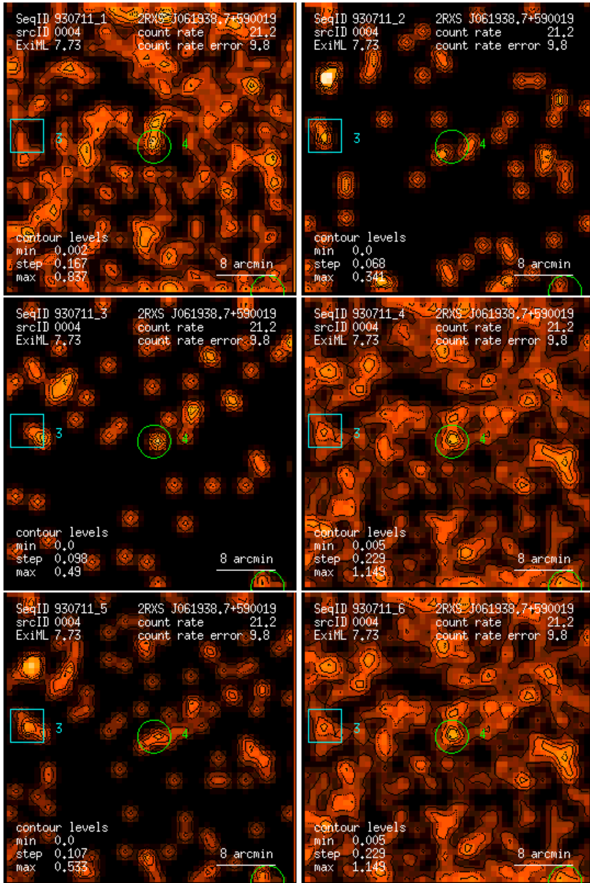
Figure 4: RASS 930711: detection 0004: band rate images, Gaussian filter: (1) PSPC channels 11 – 41, (2) 52 – 90, (3) 91 – 201, (4) 11 – 235, (5) 52 – 201, (6) 11 – 201. Broad band rates in counts/ks. Band rate contour levels in counts/ks/arcmin 2 .
