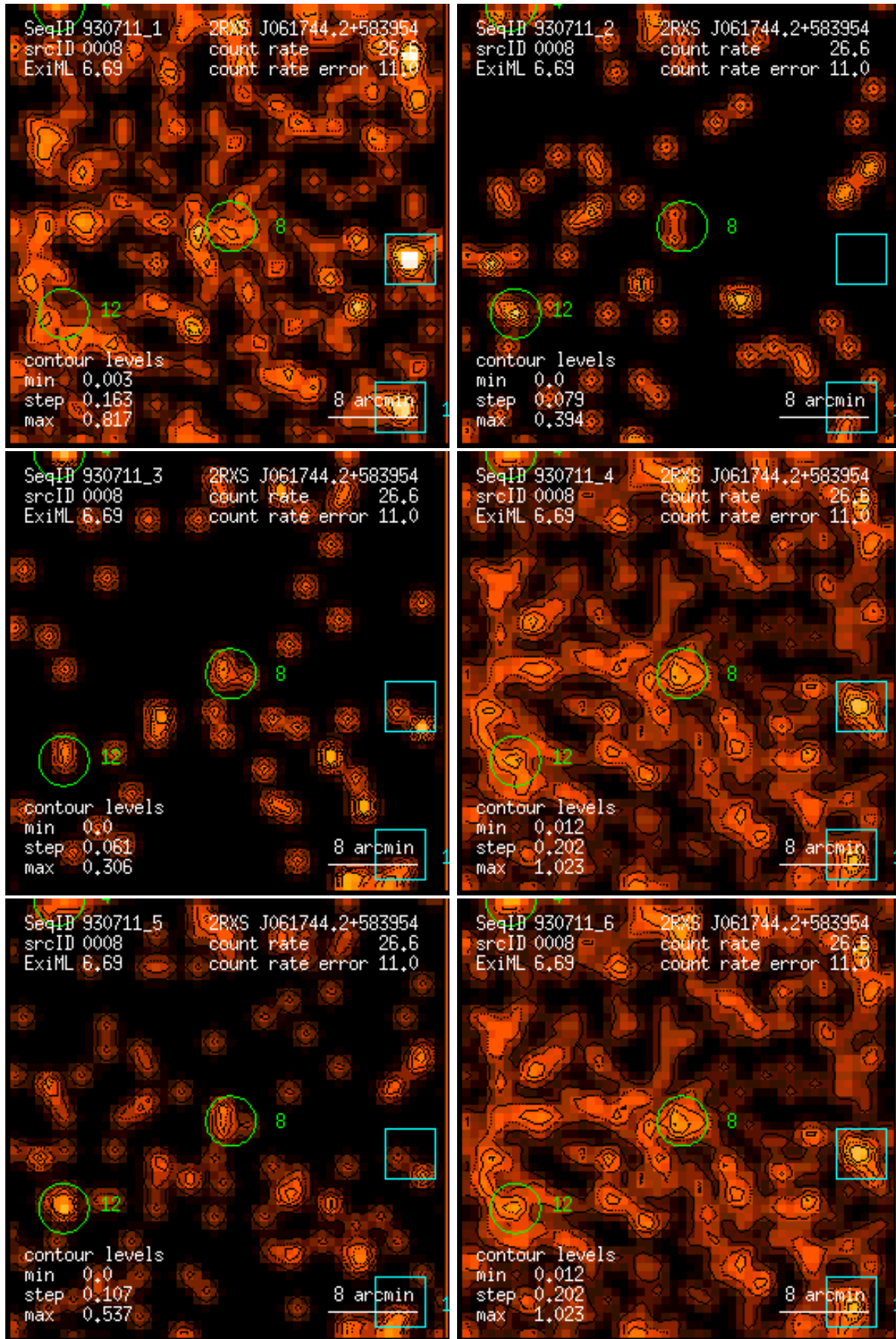
Figure 8: RASS 930711: detection 0008: band rate images, Gaussian filter: (1) PSPC channels 11 – 41, (2) 52 – 90, (3) 91 – 201, (4) 11 – 235, (5) 52 – 201, (6) 11 – 201. Broad band rates in counts/ks. Band rate contour levels in counts/ks/arcmin 2 .
