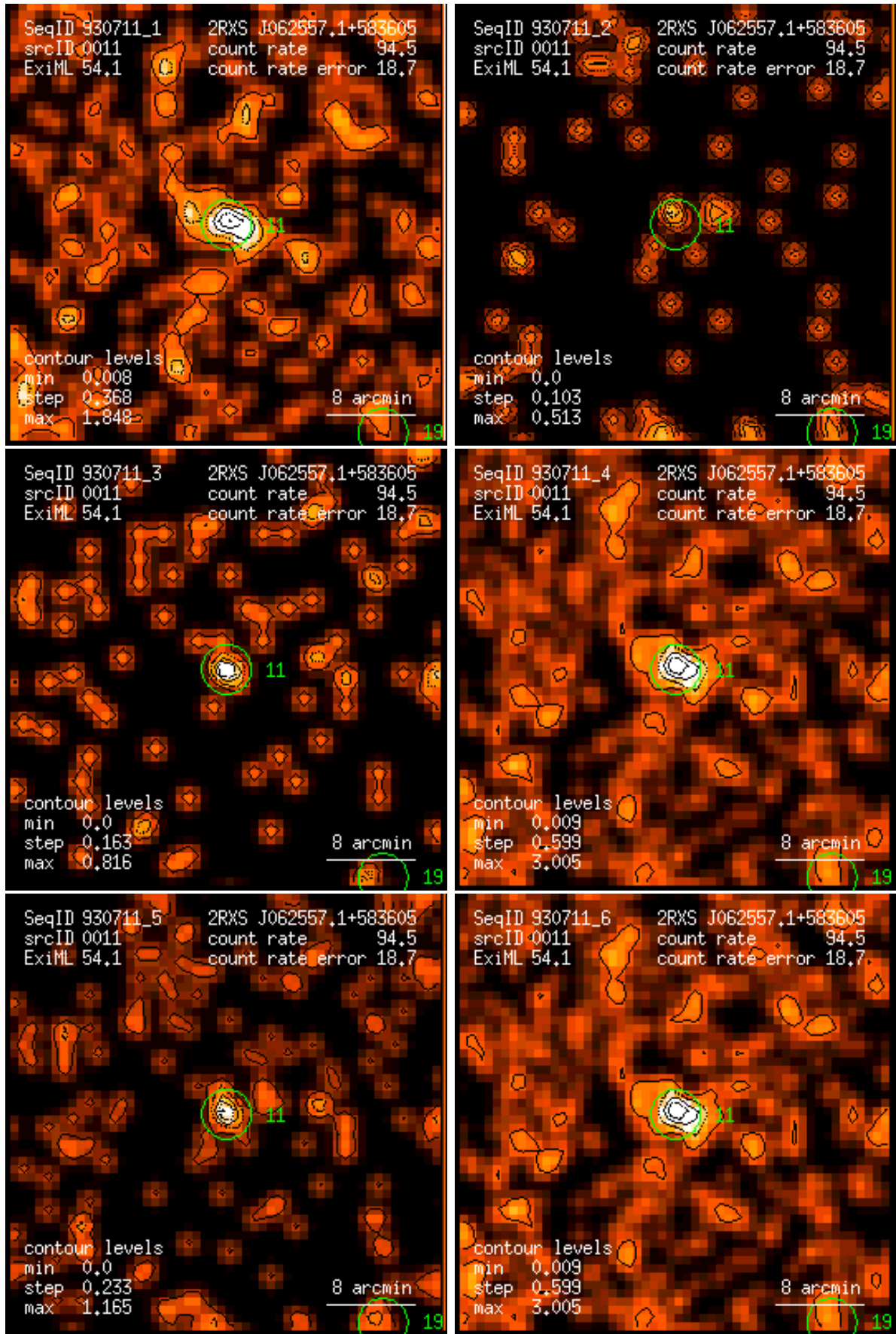
Figure 11: RASS 930711: detection 0011: band rate images, Gaussian filter: (1) PSPC channels 11 – 41, (2) 52 – 90, (3) 91 – 201, (4) 11 – 235, (5) 52 – 201, (6) 11 – 201. Broad band rates in counts/ks. Band rate contour levels in counts/ks/arcmin 2 .
