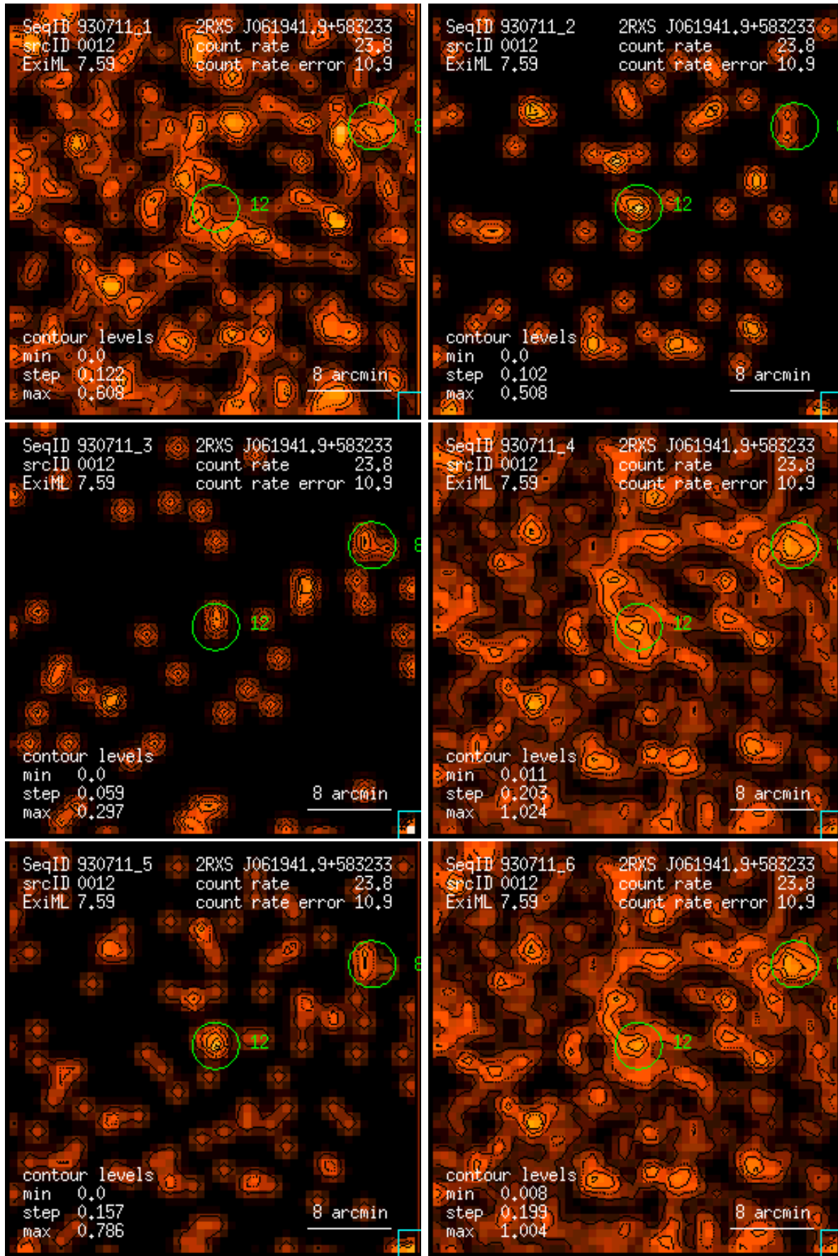
Figure 12: RASS 930711: detection 0012: band rate images, Gaussian filter: (1) PSPC channels 11 – 41, (2) 52 – 90, (3) 91 – 201, (4) 11 – 235, (5) 52 – 201, (6) 11 – 201. Broad band rates in counts/ks. Band rate contour levels in counts/ks/arcmin 2 .
