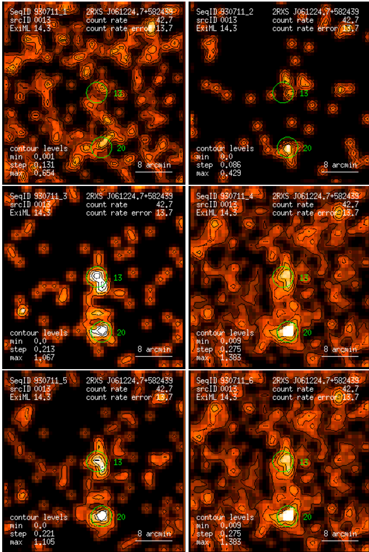
Figure 13: RASS 930711: detection 0013: band rate images, Gaussian filter: (1) PSPC channels 11 – 41, (2) 52 – 90, (3) 91 – 201, (4) 11 – 235, (5) 52 – 201, (6) 11 – 201. Broad band rates in counts/ks. Band rate contour levels in counts/ks/arcmin 2 .
