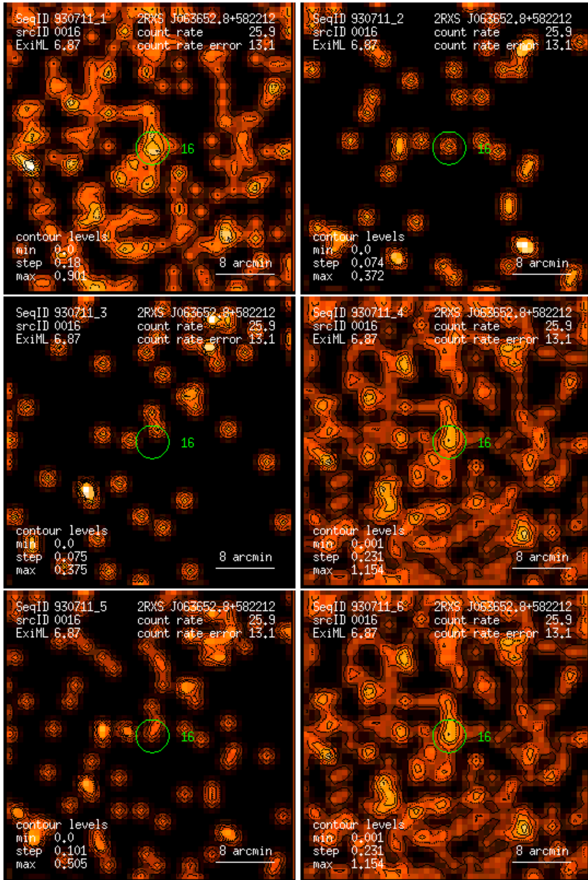
Figure 16: RASS 930711: detection 0016: band rate images, Gaussian filter: (1) PSPC channels 11 – 41, (2) 52 – 90, (3) 91 – 201, (4) 11 – 235, (5) 52 – 201, (6) 11 – 201. Broad band rates in counts/ks. Band rate contour levels in counts/ks/arcmin 2 .
