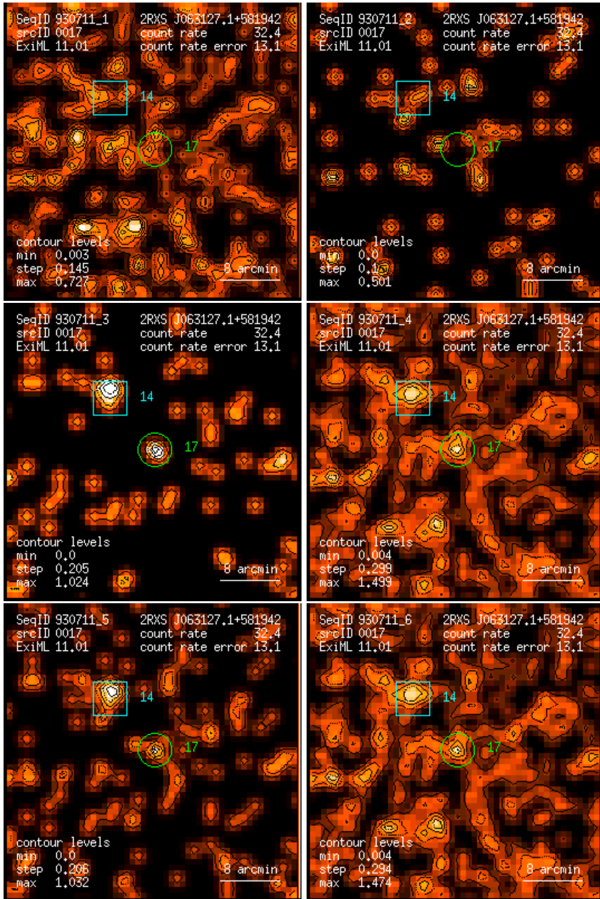
Figure 17: RASS 930711: detection 0017: band rate images, Gaussian filter: (1) PSPC channels 11 – 41, (2) 52 – 90, (3) 91 – 201, (4) 11 – 235, (5) 52 – 201, (6) 11 – 201. Broad band rates in counts/ks. Band rate contour levels in counts/ks/arcmin 2 .
