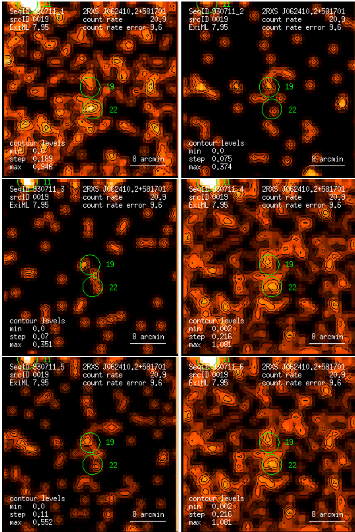
Figure 19: RASS 930711: detection 0019: band rate images, Gaussian filter: (1) PSPC channels 11 – 41, (2) 52 – 90, (3) 91 – 201, (4) 11 – 235, (5) 52 – 201, (6) 11 – 201. Broad band rates in counts/ks. Band rate contour levels in counts/ks/arcmin 2 .
