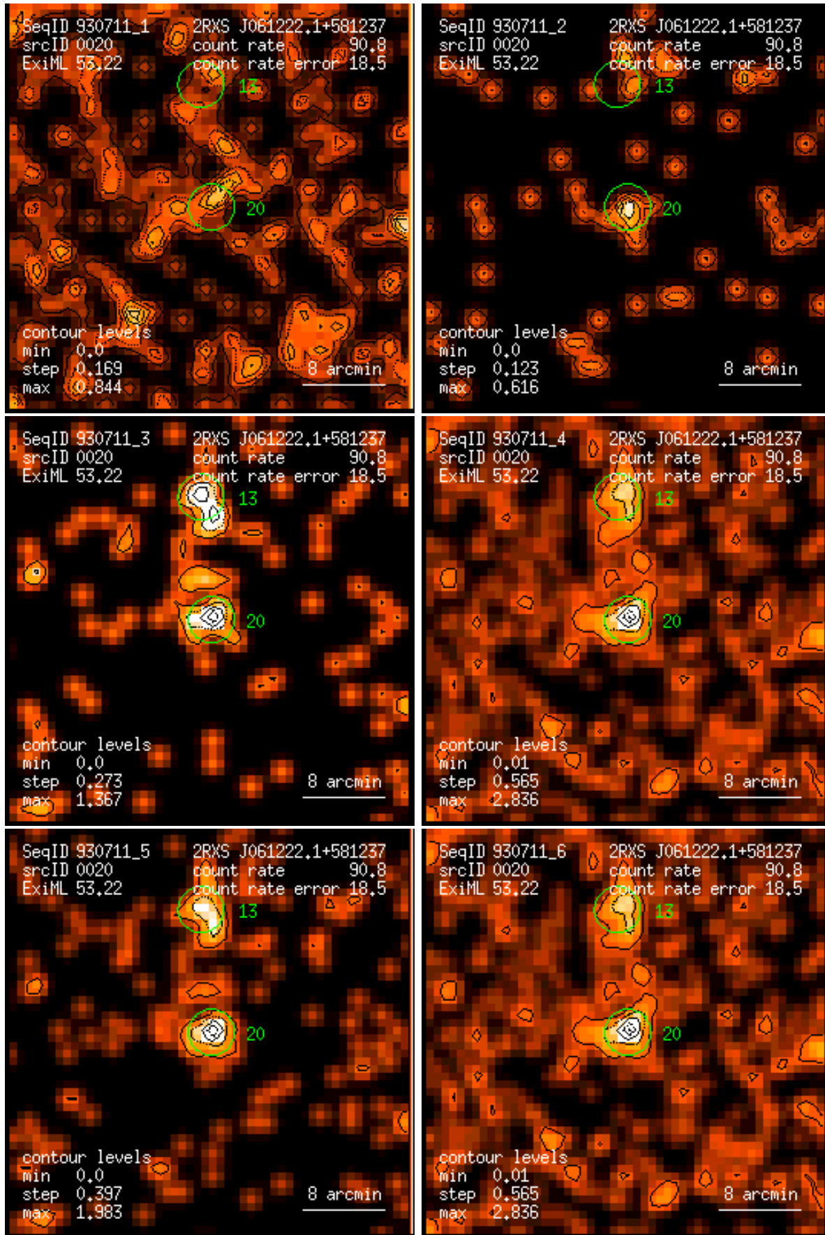
Figure 20: RASS 930711: detection 0020: band rate images, Gaussian filter: (1) PSPC channels 11 – 41, (2) 52 – 90, (3) 91 – 201, (4) 11 – 235, (5) 52 – 201, (6) 11 – 201. Broad band rates in counts/ks. Band rate contour levels in counts/ks/arcmin 2 .
